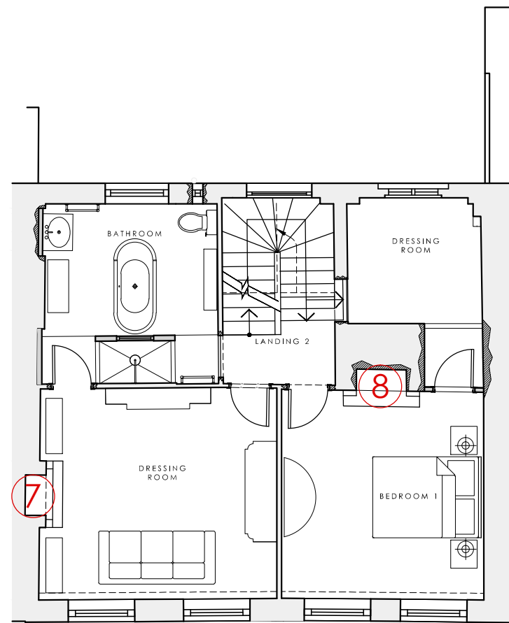
Second Floor
