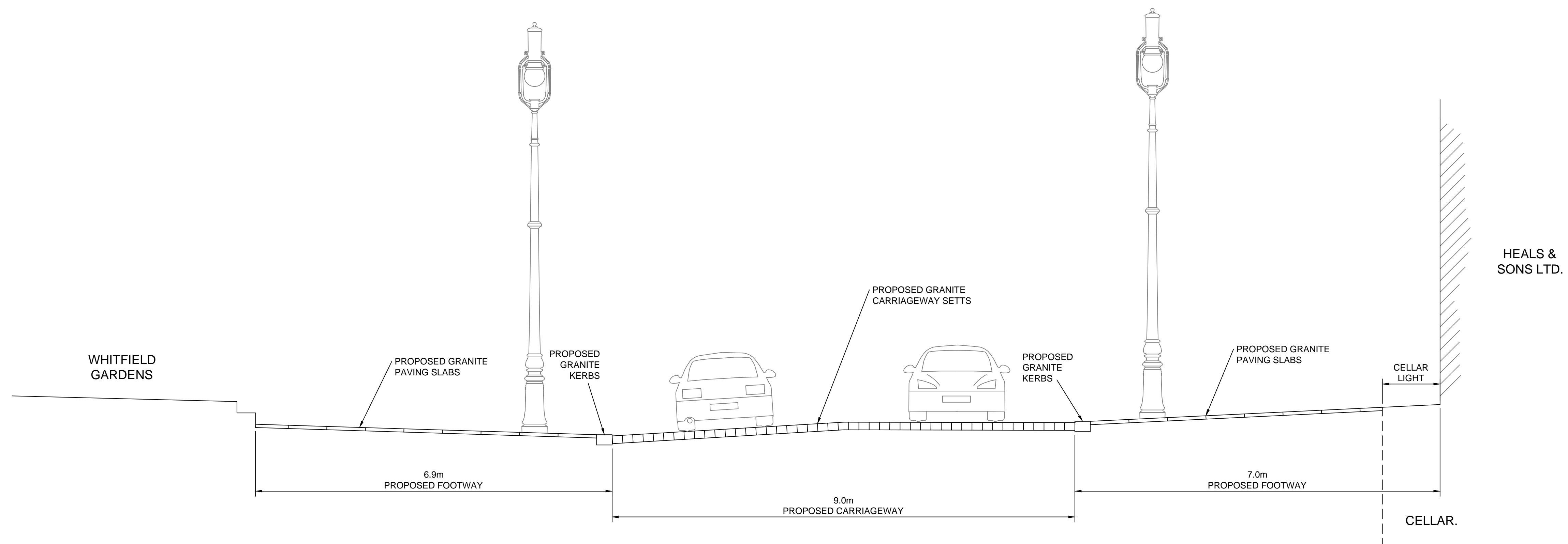
PROPOSED LAYOUT (OUT OF RESTRICTED HOURS) SECTION A-A
