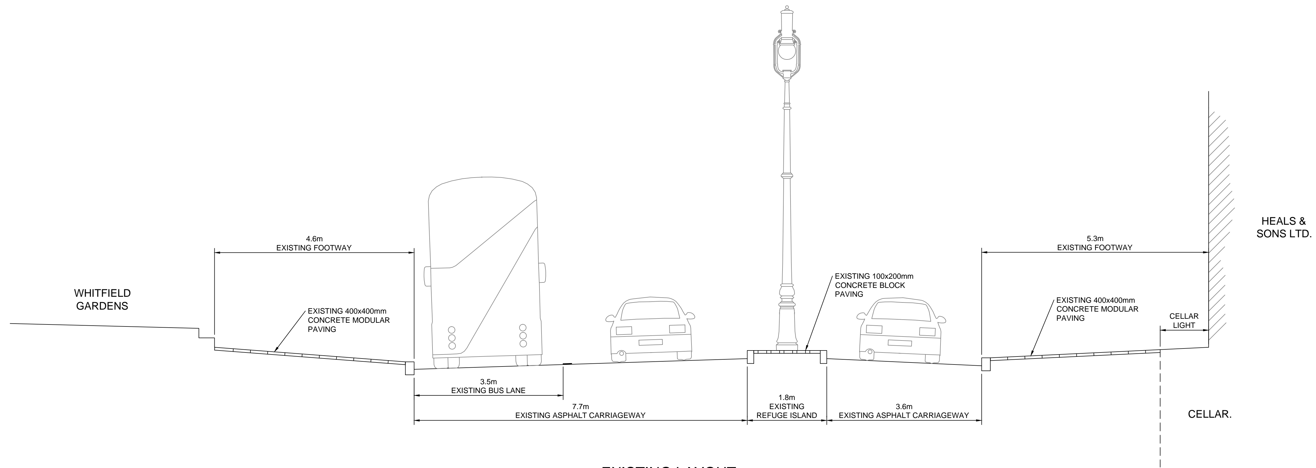
EXISTING LAYOUT SECTION A-A
