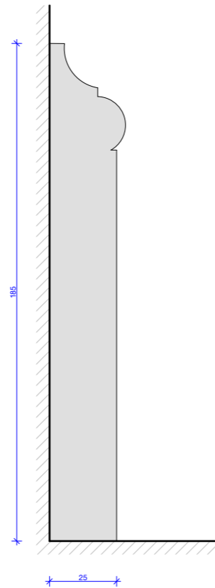
1:2 New cornice Full brooks of England : C20 - Plane Cove Cornice
