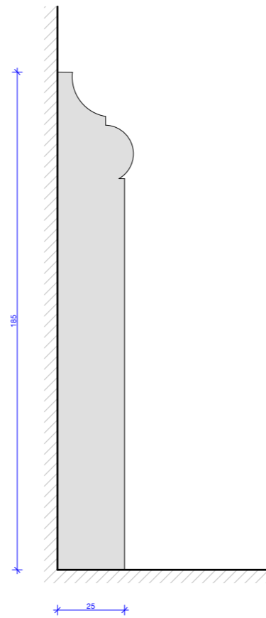
1:2 Skirting proposed - to match 3rd floor skirting
