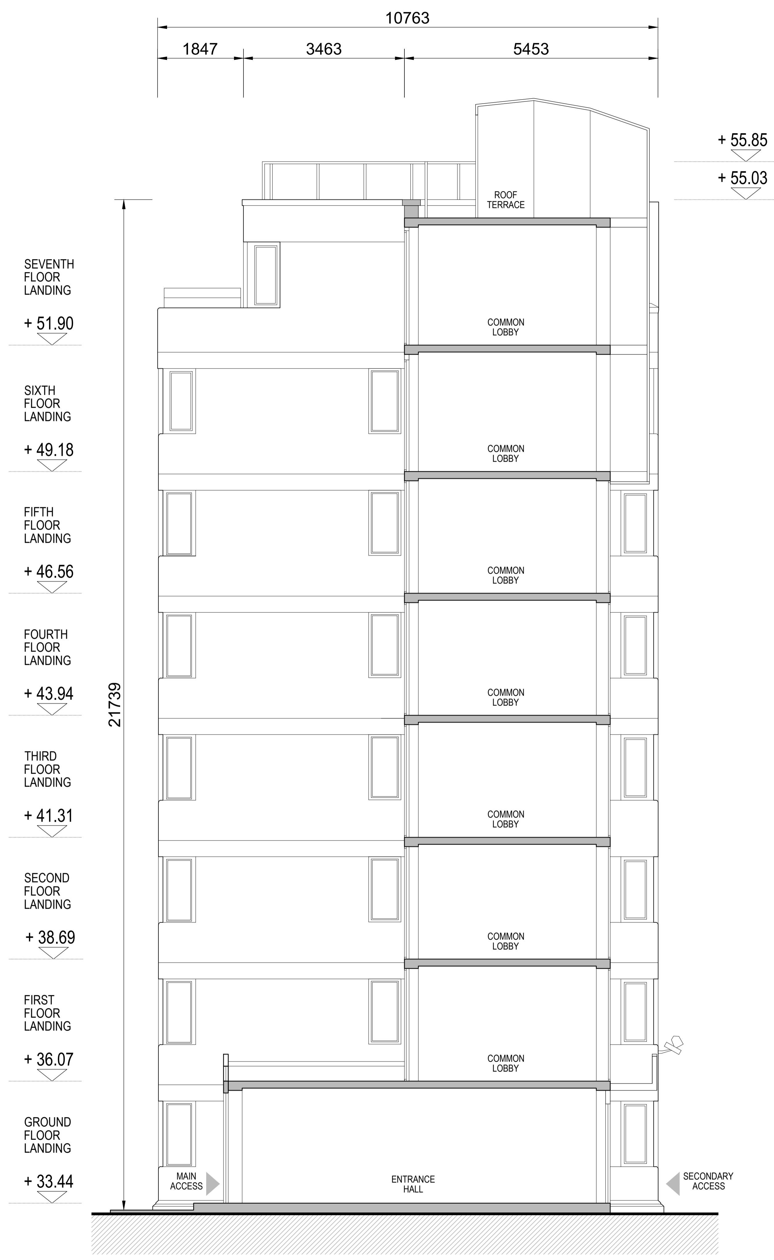
1 SHORT SECTION 1 1:50
