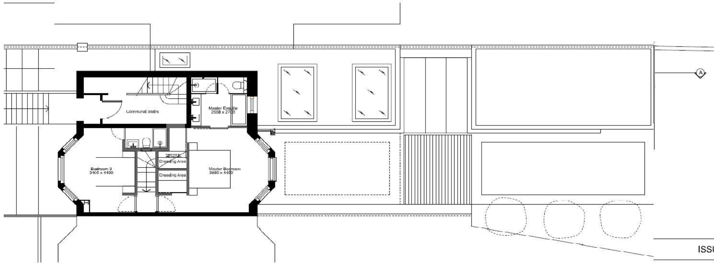
Raised Ground Floor Plan
