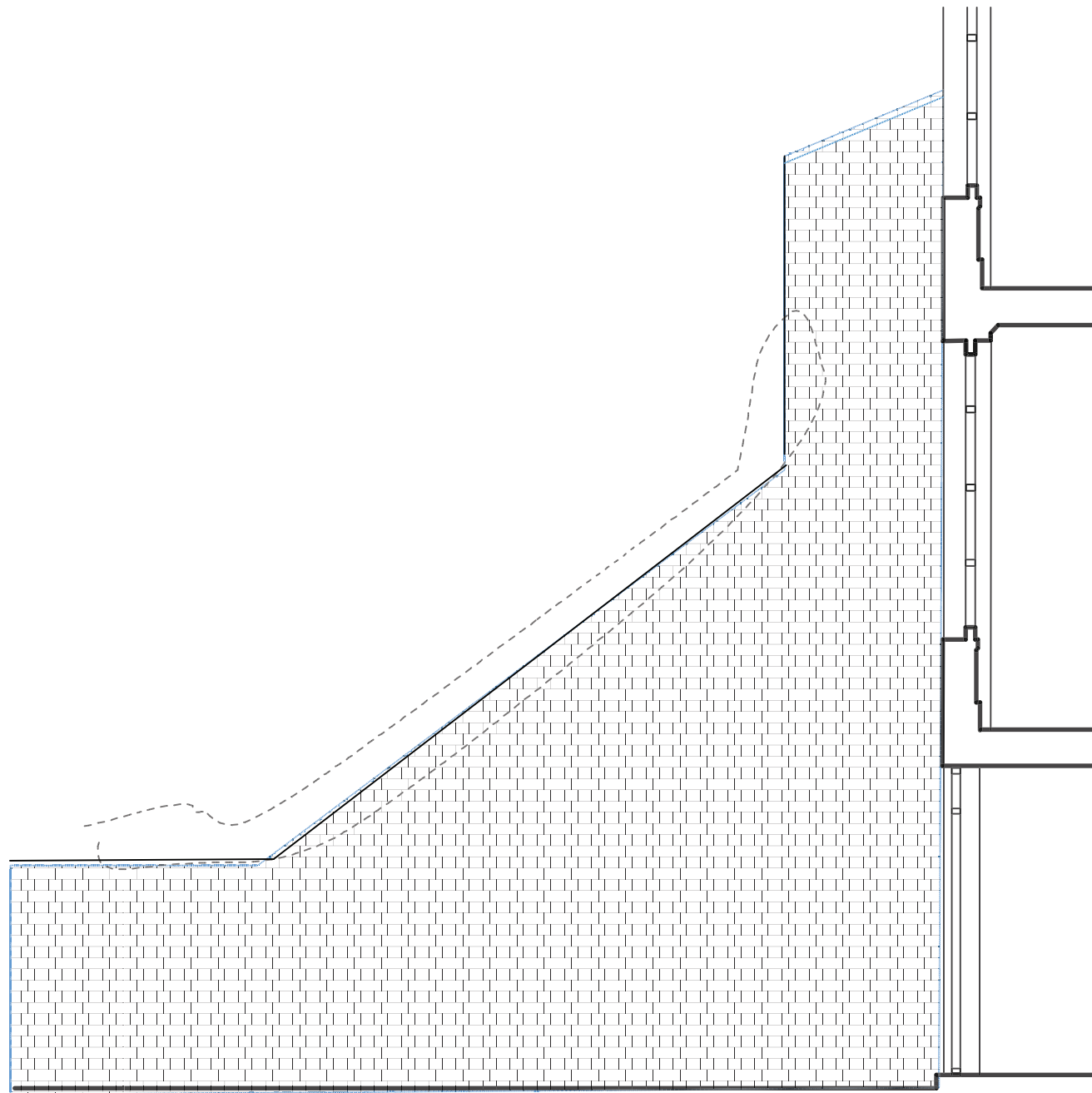
SECTION G-G
