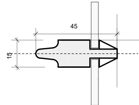
Typical section through glazing bar as existing at 11 Gloucester Crescent. SCALE 1:1 @A3
