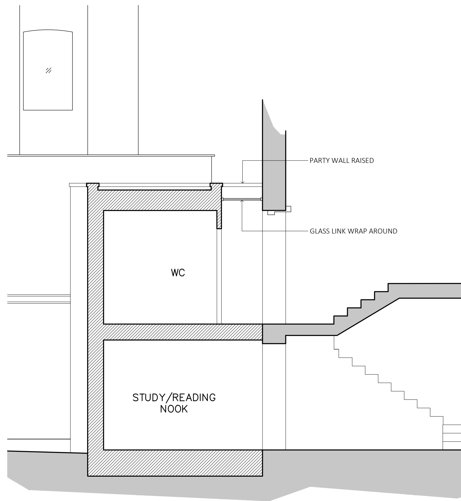
SECTION B-B
