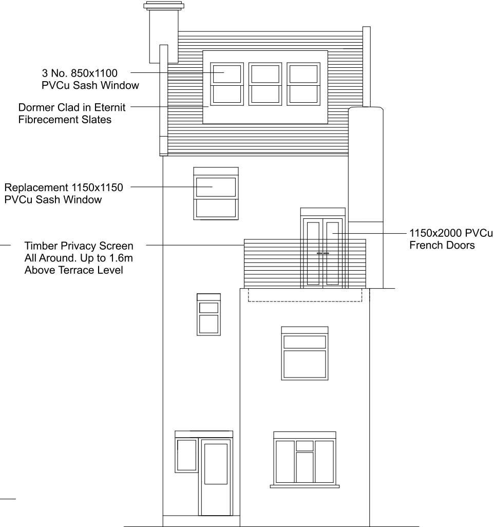
REAR ELEVATION AS PROPOSED
