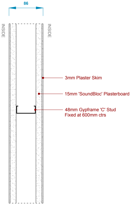
02 Type A Plan
