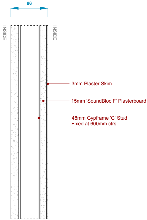
05 Type C Section
