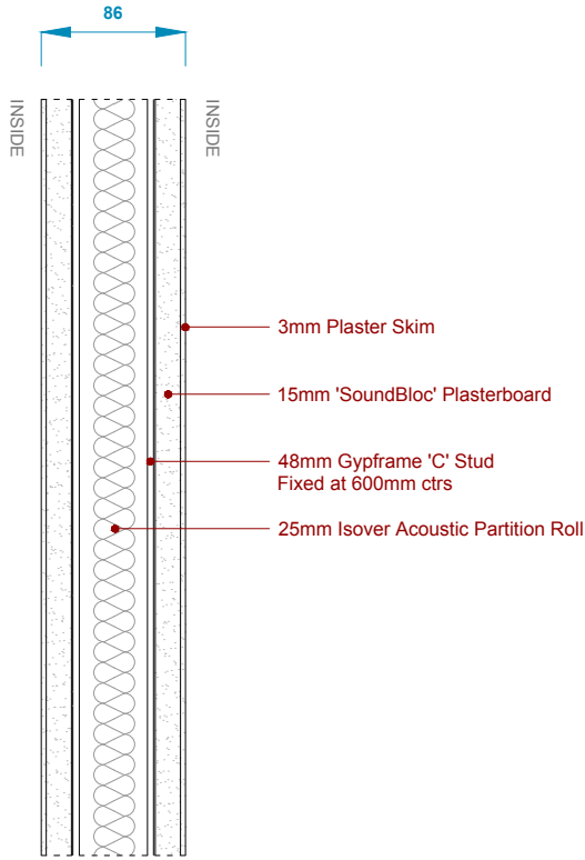
03 Type B Section
