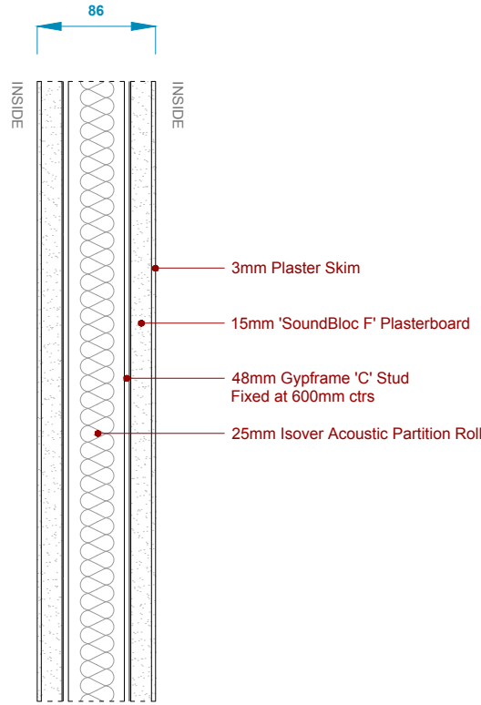
07 Type D Section
