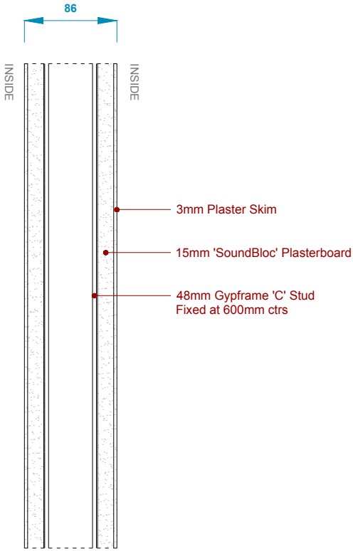
01 Type A Section
