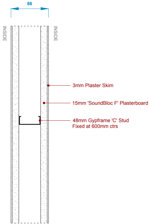
06 Type C Plan
