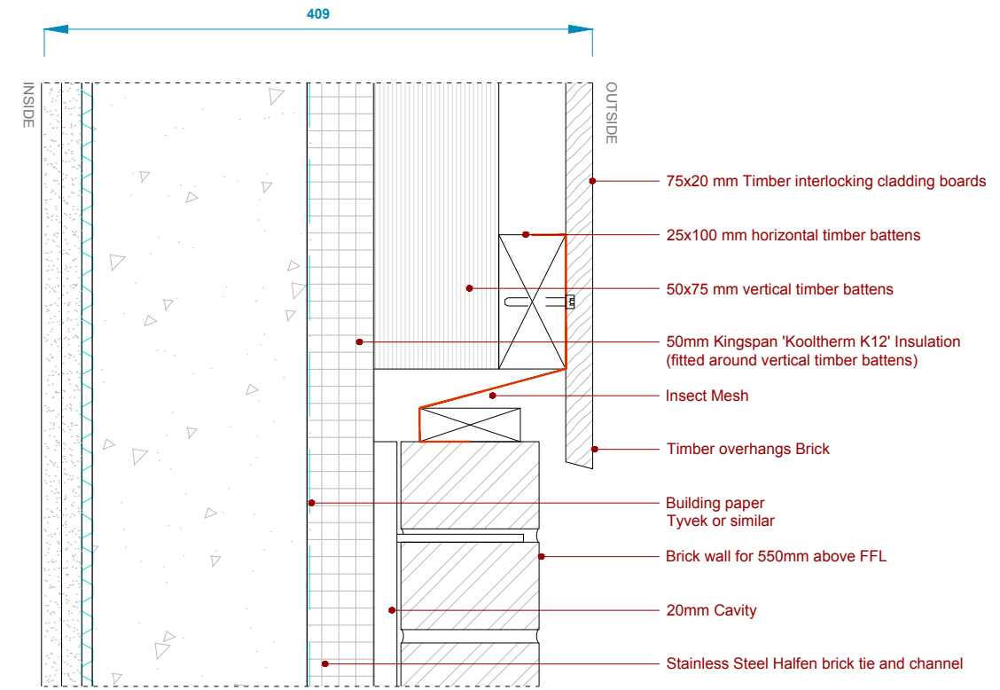
03 Type B : Brick plinth / Timber Section
