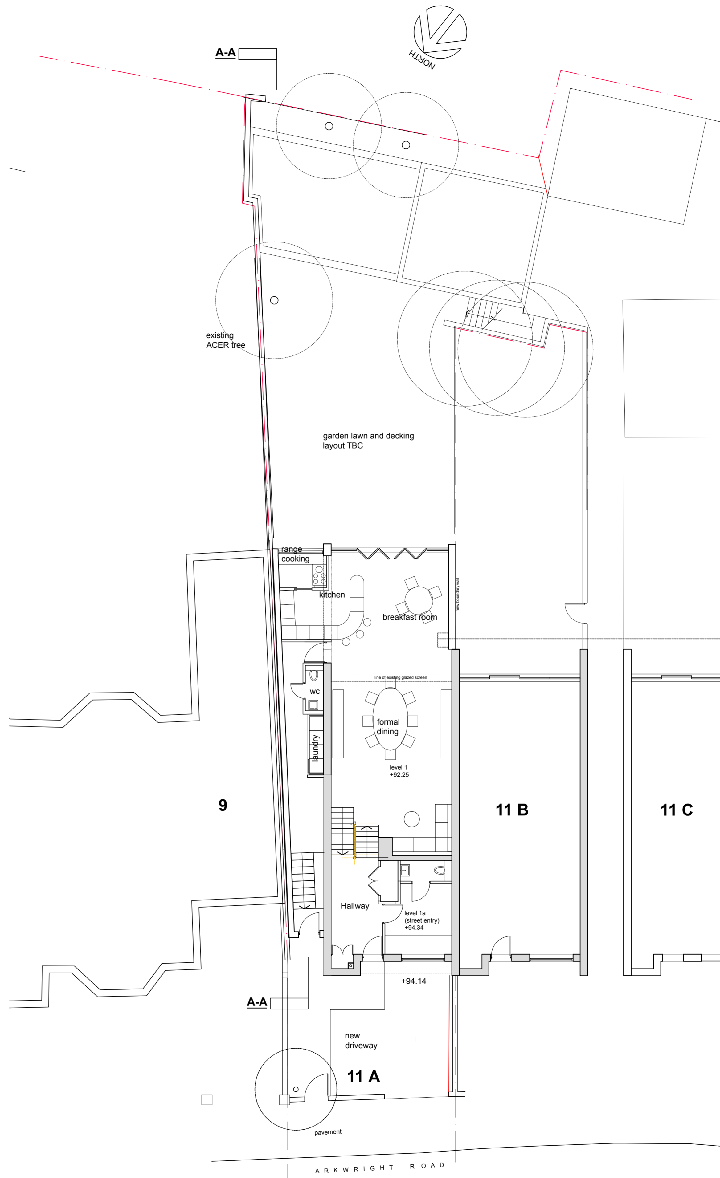
PROPOSED GROUND FLOOR Scale 1:100
