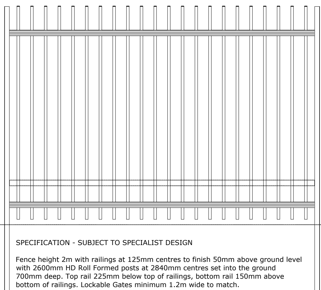
2M HIGH BLACK STEEL RAILINGS
