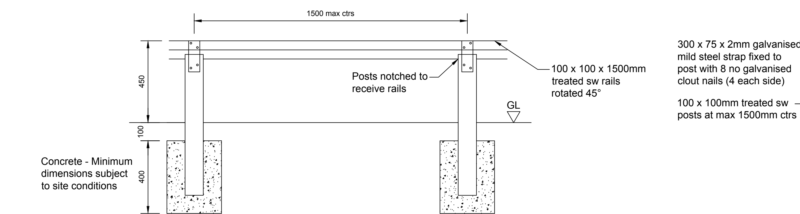
450mm Knee high Post & Rail Elevation
