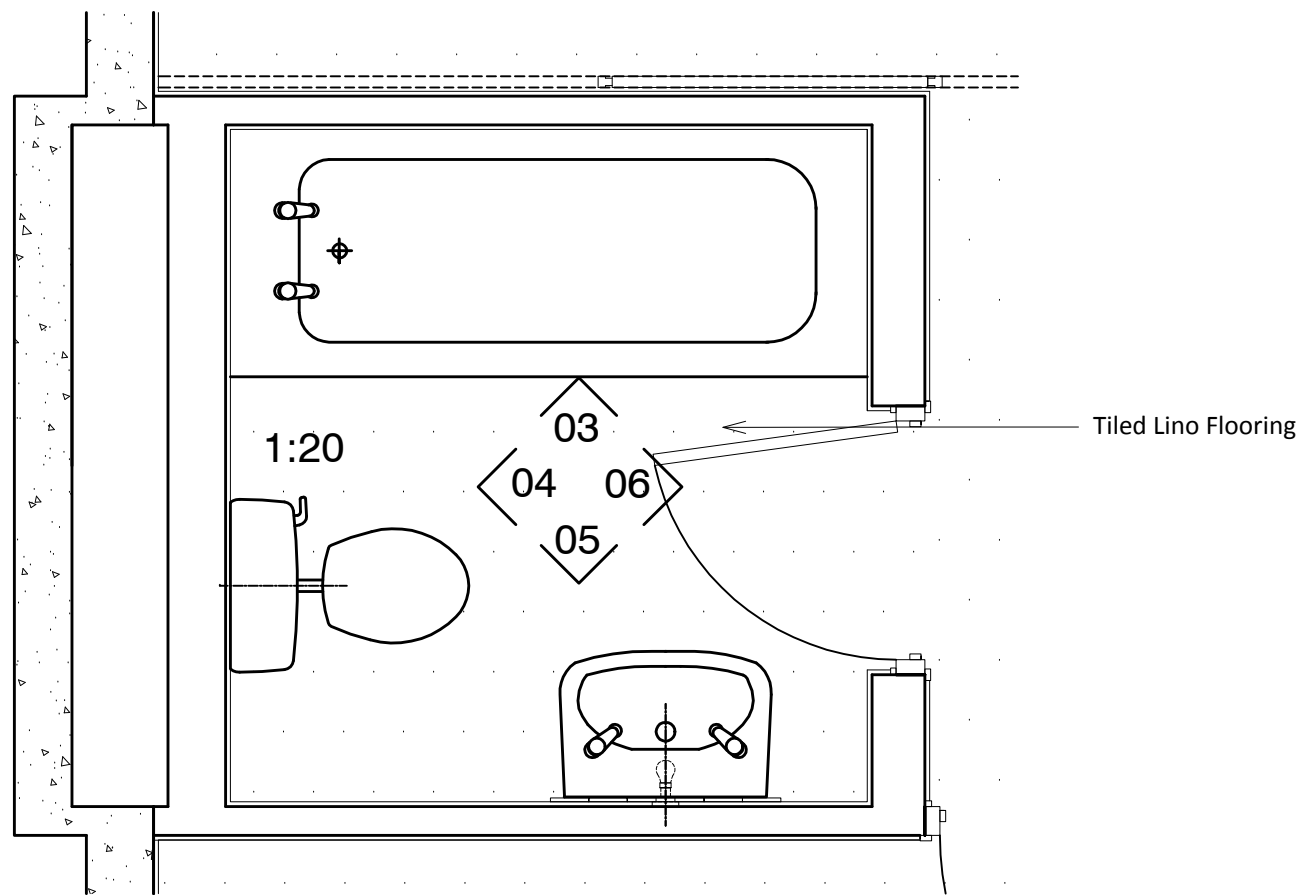
01 Ground Floor Bathroom Plan 207 1:20
