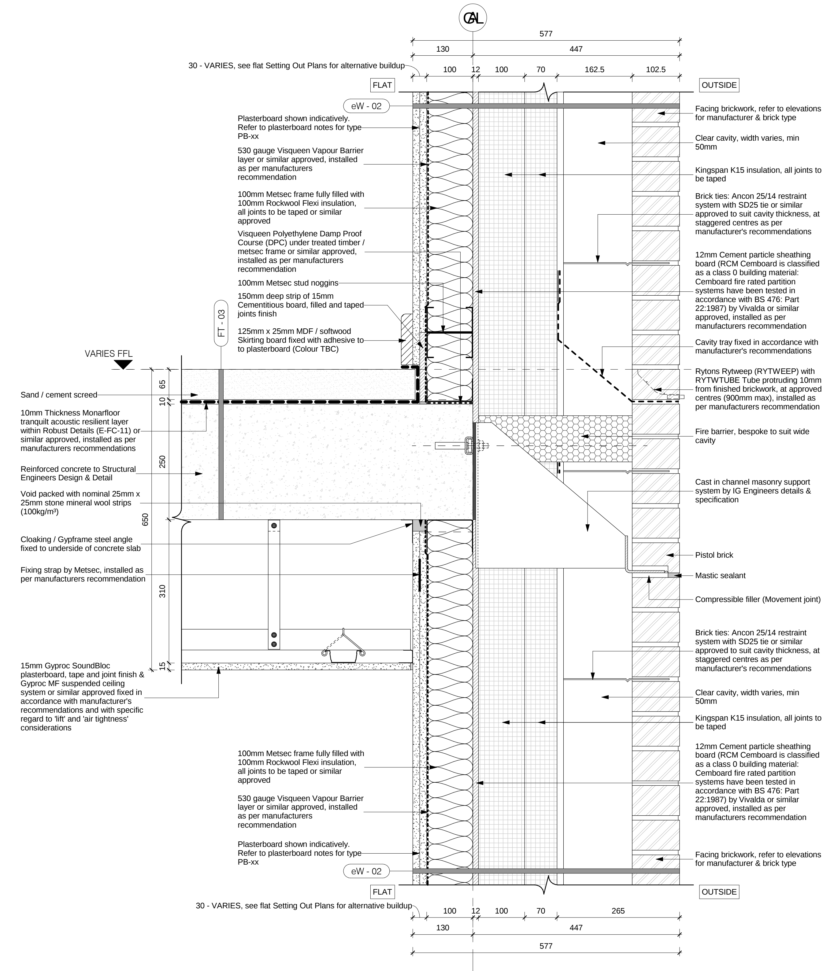
Typical Section of External Wall with Cast in channel masonry support system (Stretcher Bond) & Separating Floor between Flat to Flat
