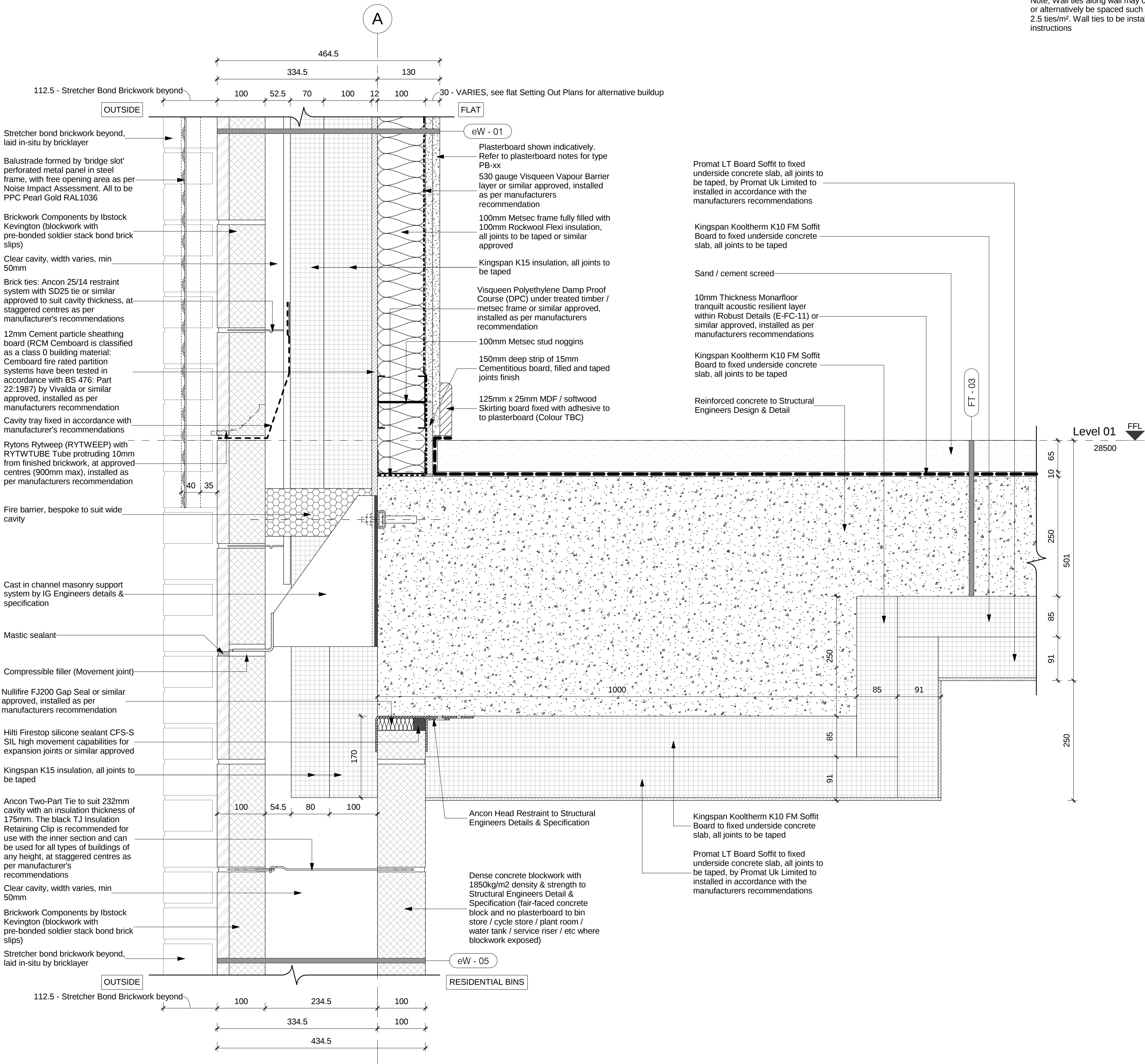
Section of External Wall with Cast in channel masonry support system (Soldier-Course Stack Bond), Slab Edge Detail & Separating Floor between Residential Bins to Flat
