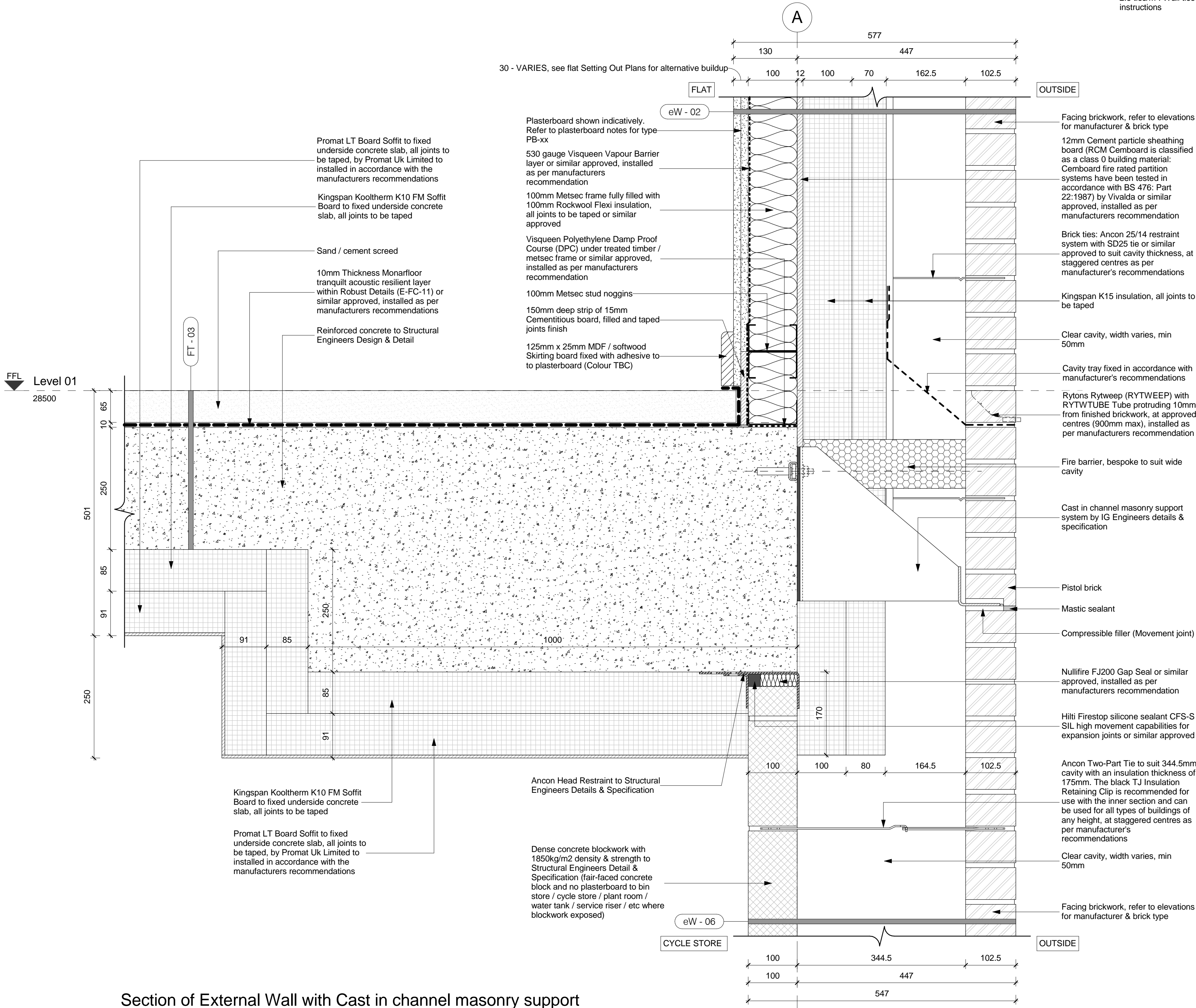
Section of External Wall with Cast in channel masonry support system (Stretcher Bond), Slab Edge Detail & Separating Floor between Cycle Store & Flat
