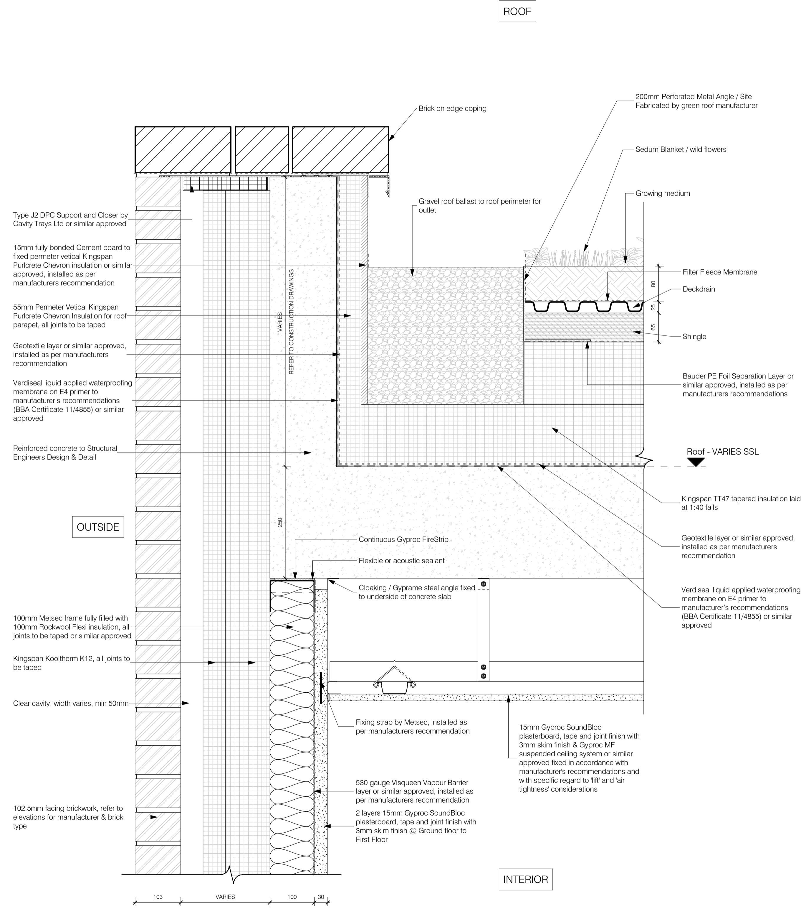
2 ROBS / VARS upper roof Scale: 1:5
