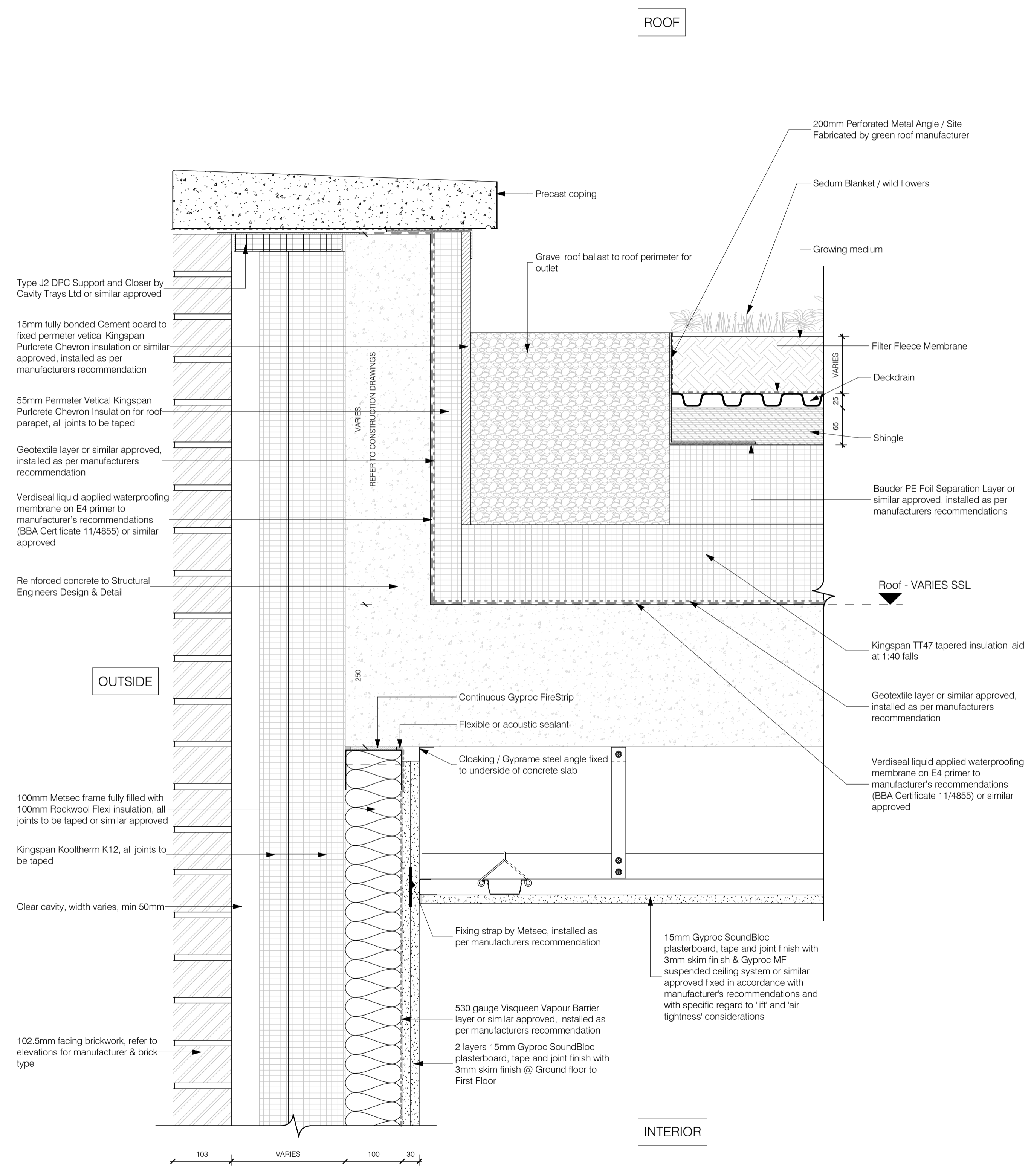
2 DCH lower roof Scale: 1:5
