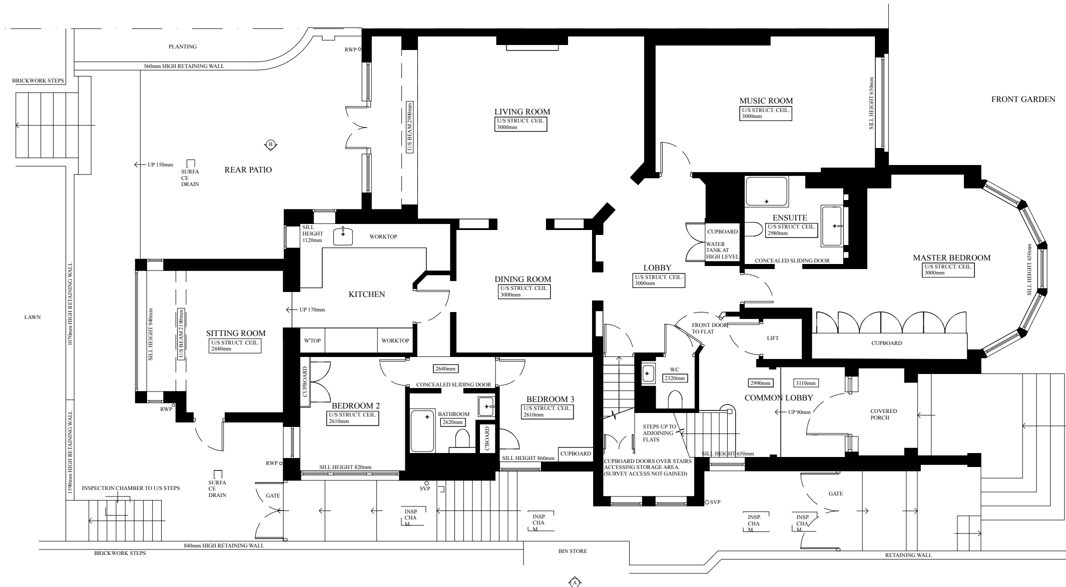
1 EXISTING GROUND FLOOR PLAN - GIA:164.7 m 2 Scale: 1:50
