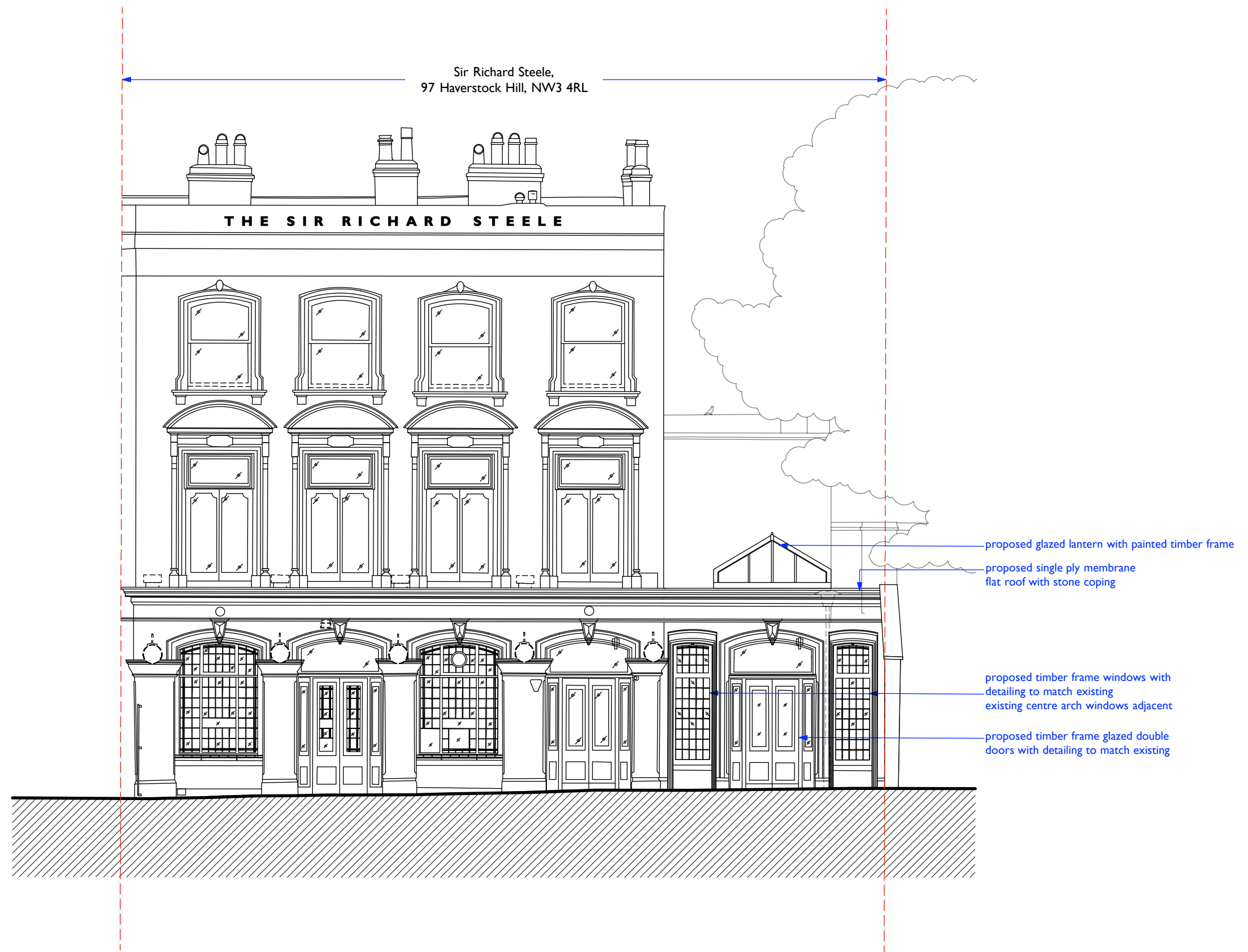
PROPOSED SIDE ELEVATION C-C
