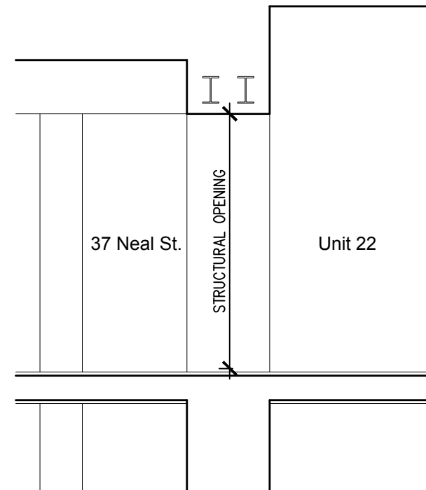
Section B-B (1:50)
