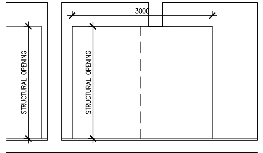
Section A-A (1:50)
