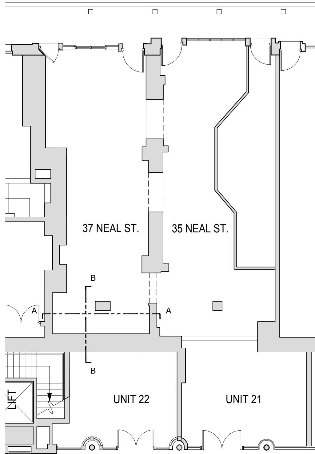
Plan (1:100)
