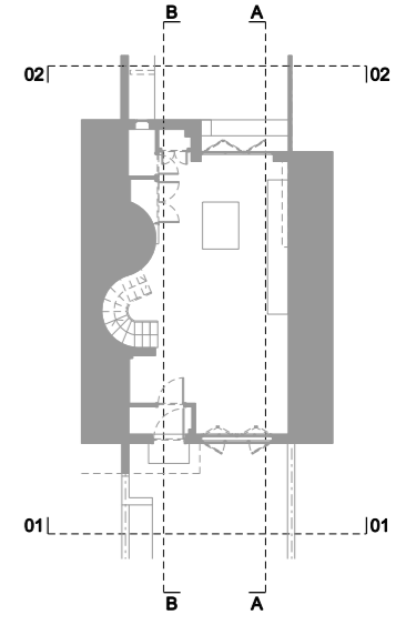
VANE CLOSE KEY PLAN
