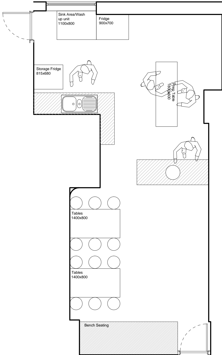
EXISTING AND PROPOSED GROUND FLOOR PLAN Scale @ 1/50
