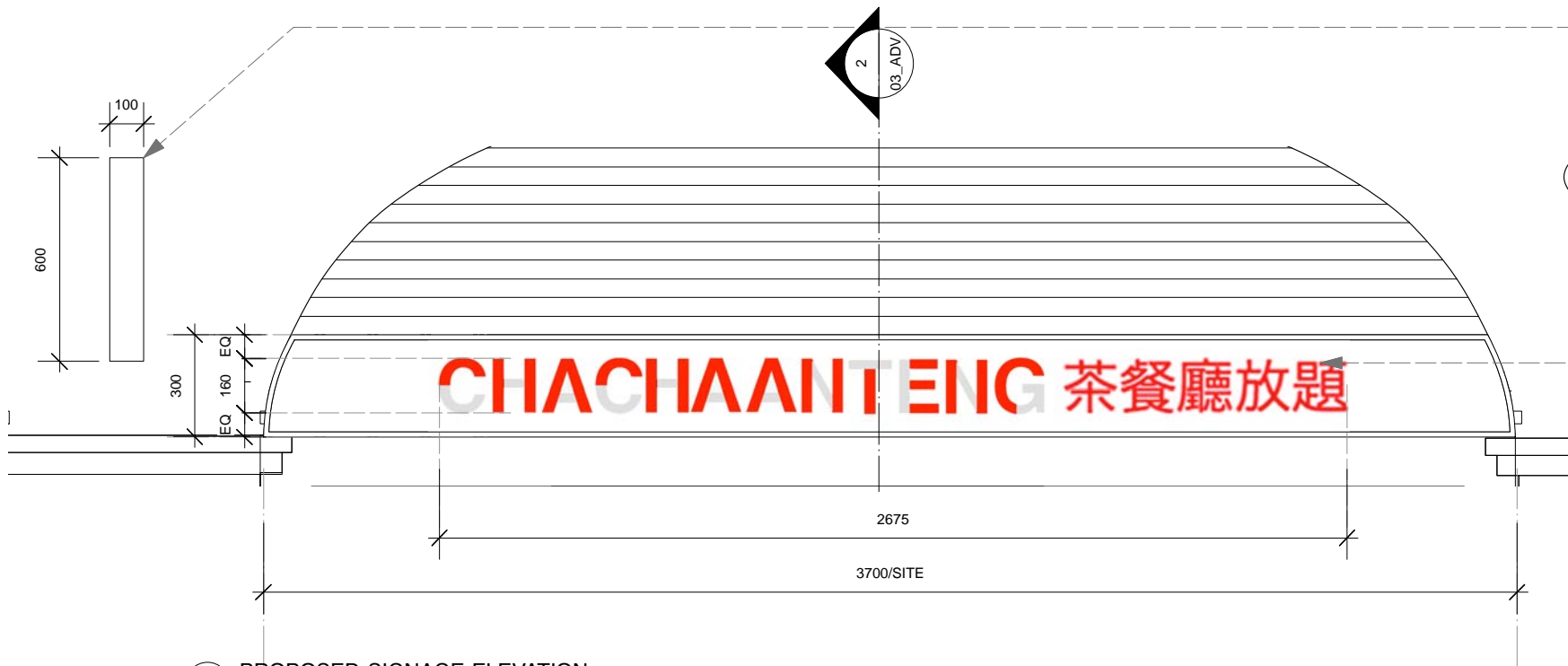
2 PROPOSED SIGNAGE ELEVATION 1:20
