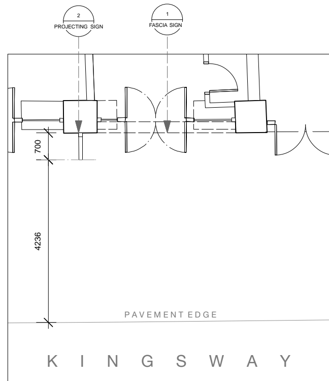
3 PROPOSED FACADE_PLAN (INC PAVEMENT) 1:100
