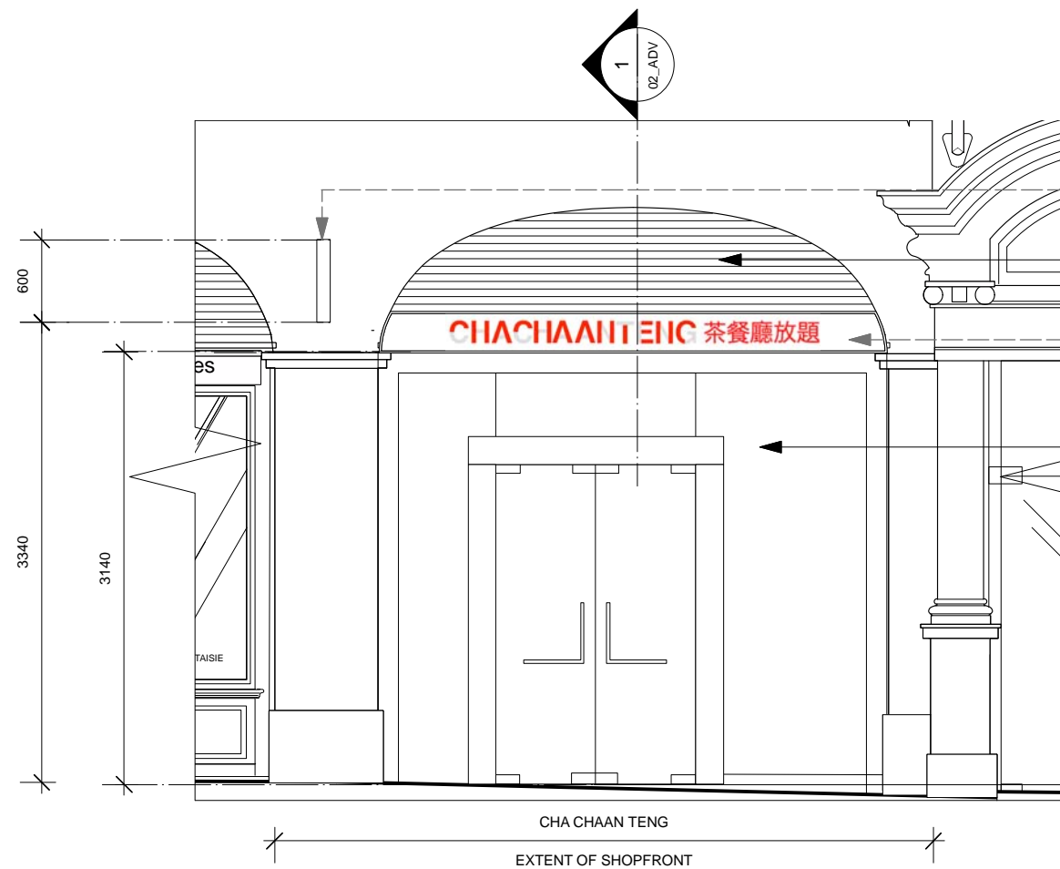
1 PROPOSED FACADE_ELEVATION A 1:50
