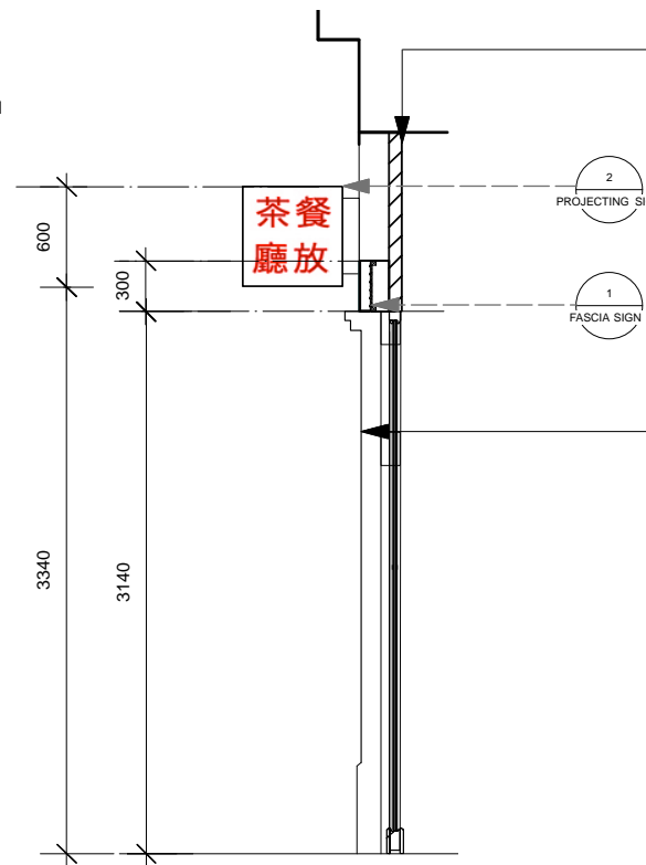
2 PROPOSED FACADE_SECTION 1 1:50
