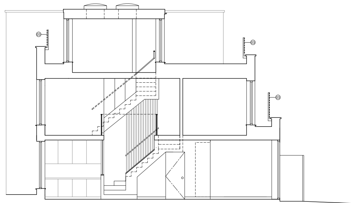
Proposed Section
