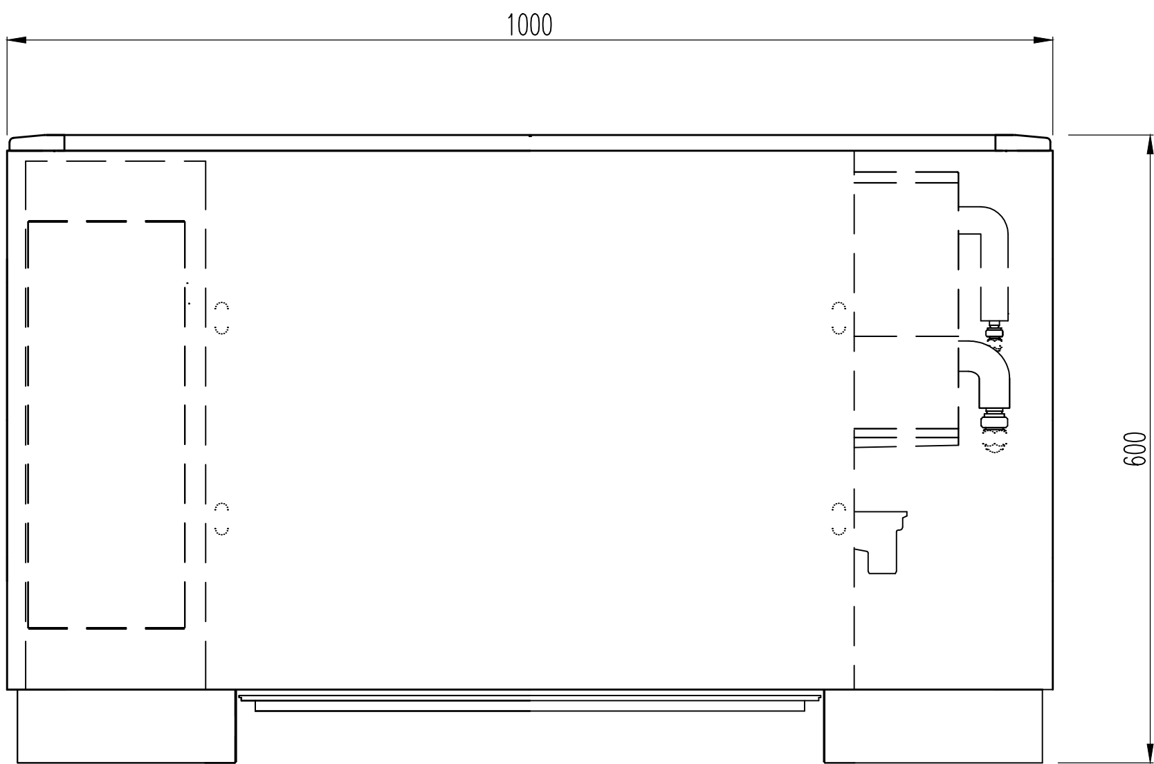
FRONT VIEW
