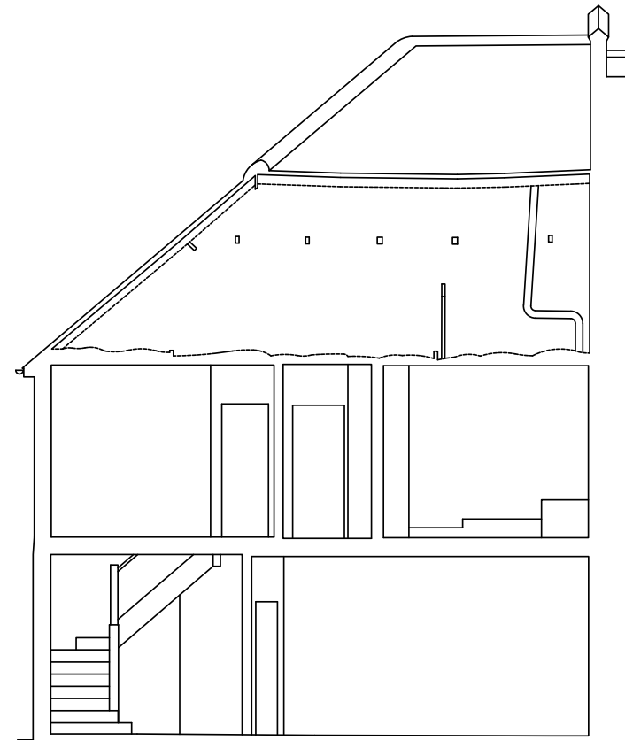
EXISTING SECTION A - A
