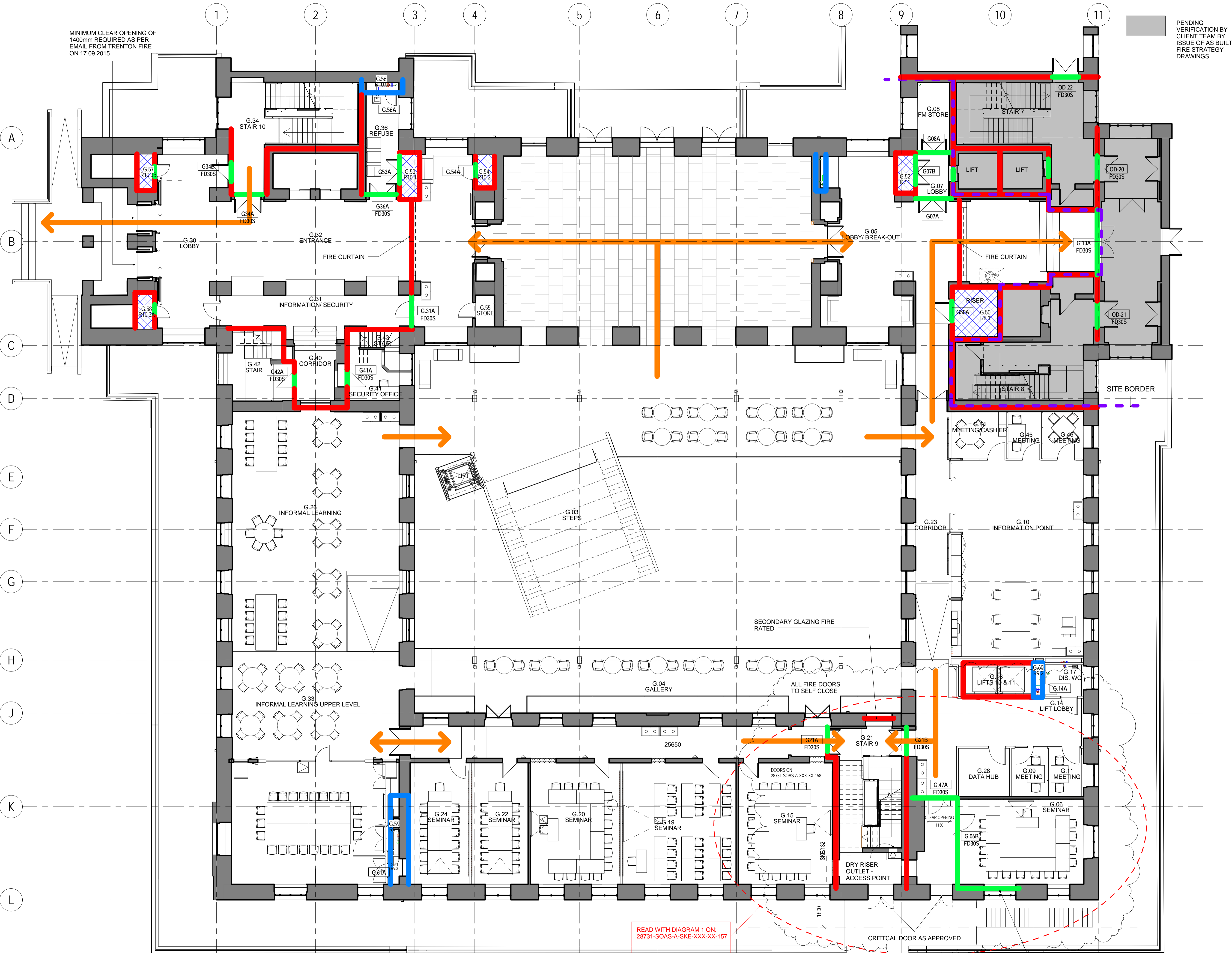
1 PROPOSED GROUND FLOOR FIRE STRATEGY PLAN 1:100
