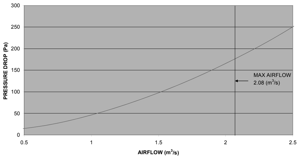
RESISTANCE AGAINST AIRFLOW ESP4500E
