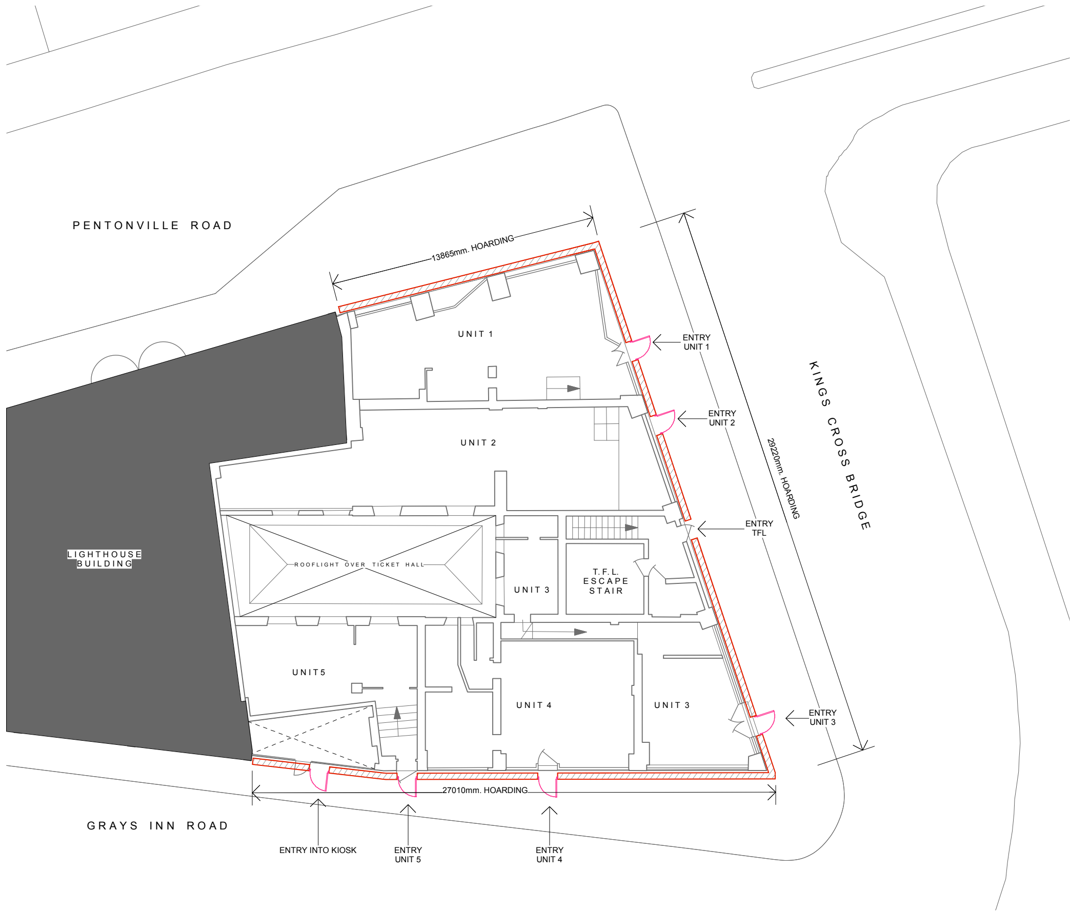
PROPOSED HOARDING GROUND FLOOR PLAN
