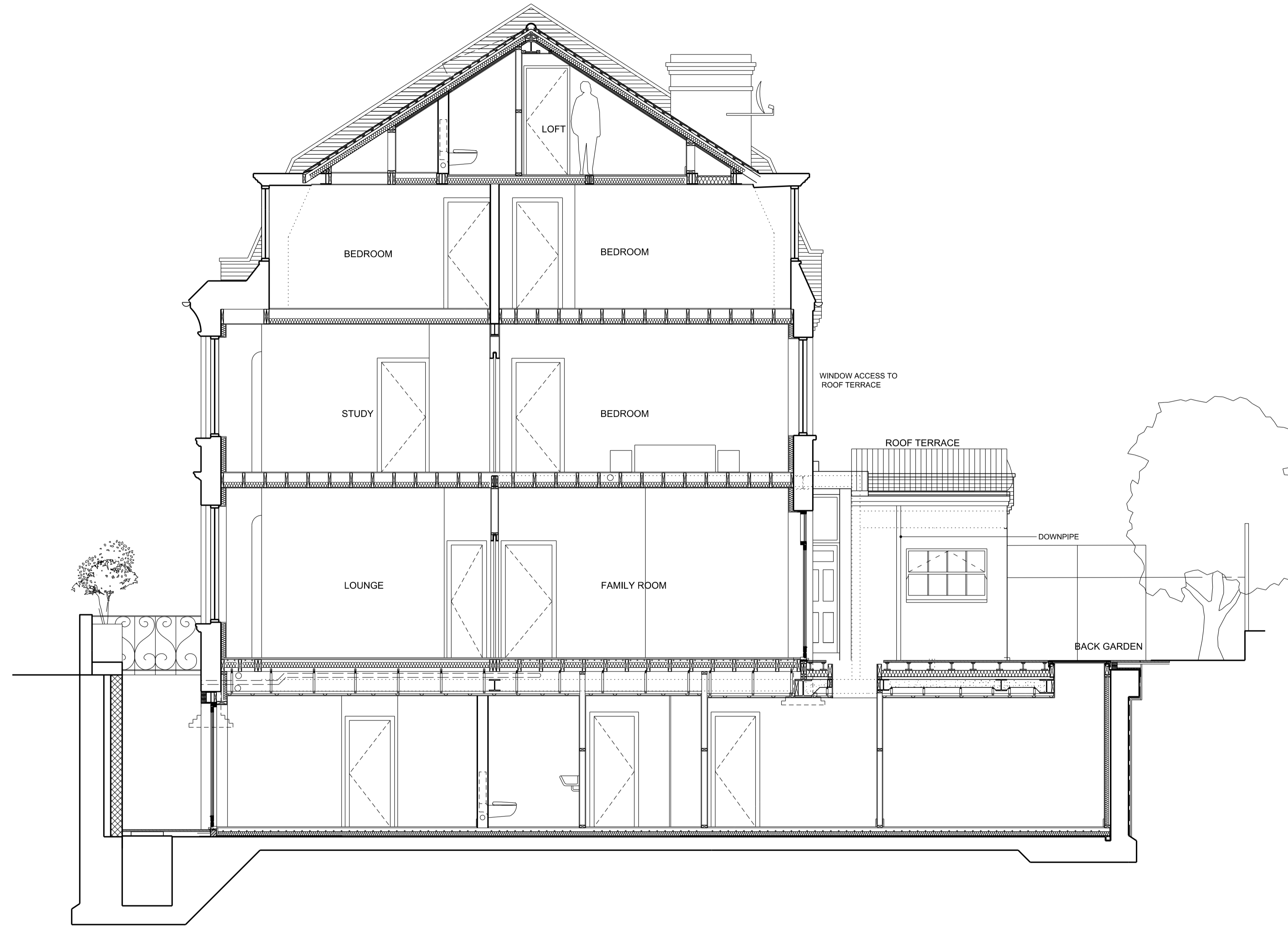
01 EXISTING CONSENTED SECTION A-A 1:50
