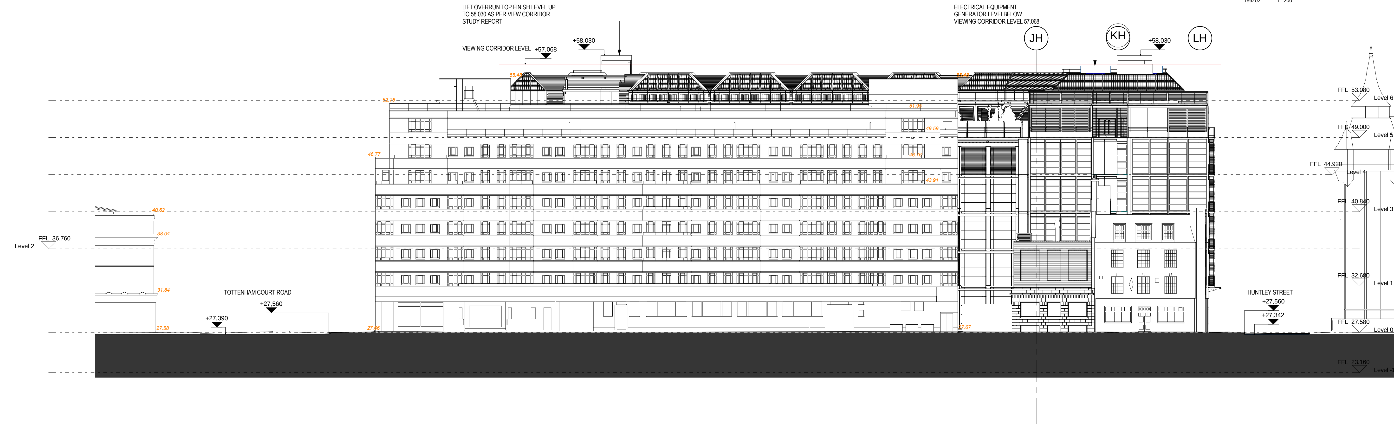
ELE-04 University Street Elevation 156202 1 : 200
