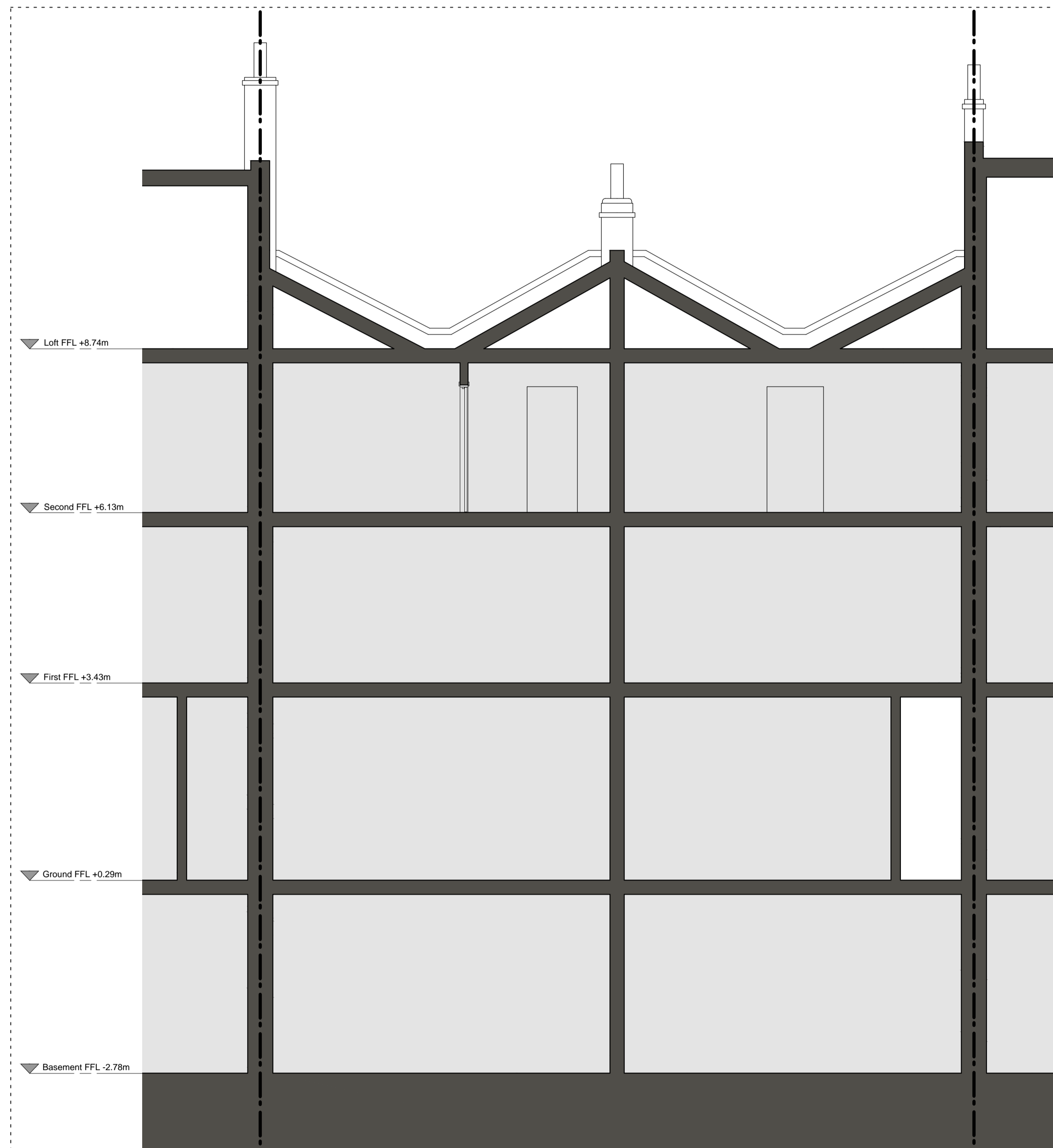
EXISTING SECTION AA
