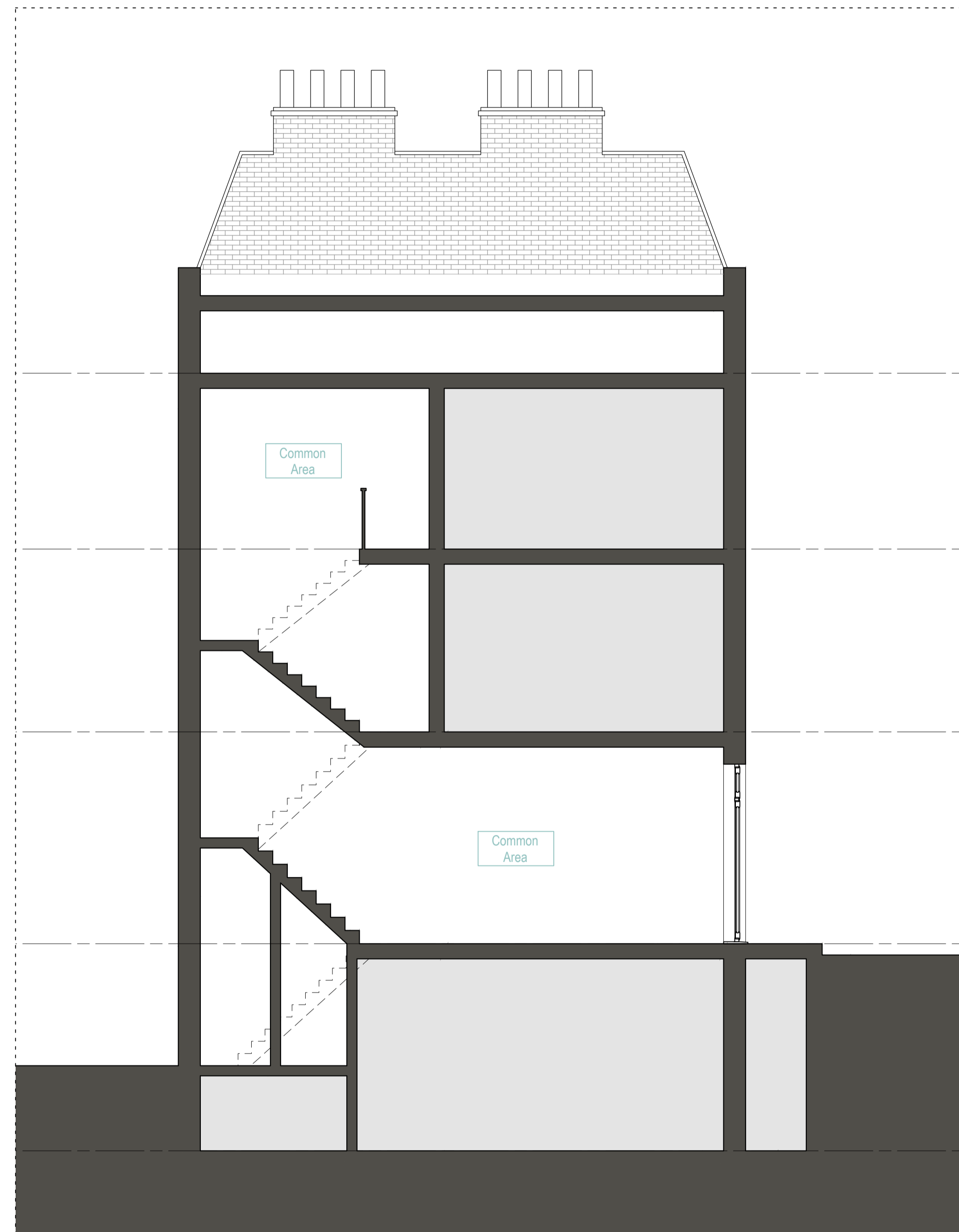
EXISTING SECTION BB
