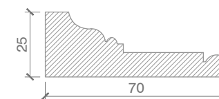
TYP. ARCHITRAVE DETAIL HIERARCHY 3 REGENCY PERIOD SCALE - 1:2
