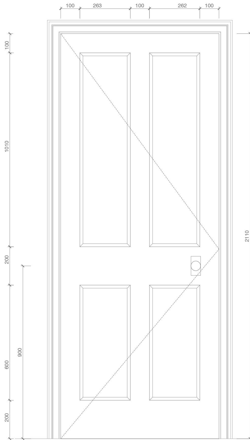
TYP. DOOR DETAIL, (FD30) HIERARCHY 3 REGENCY PERIOD, FOUR PANEL DOOR SCALE - 1:10
