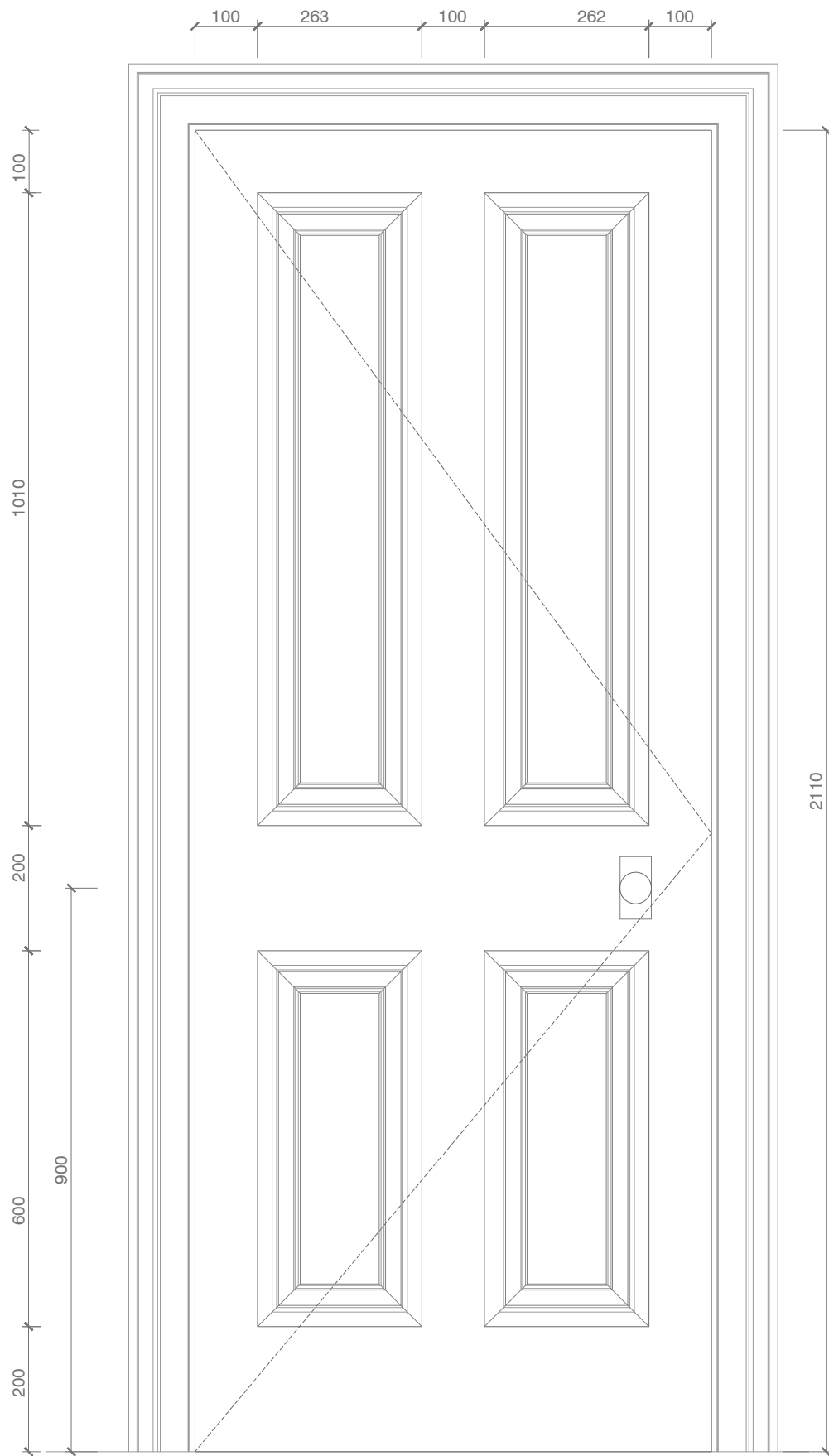
TYP. DOOR DETAIL, (FD30) HIERARCHY 2 REGENCY PERIOD, FOUR PANEL DOOR SCALE - 1:10
