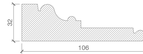
TYP. ARCHITRAVE DETAIL HIERARCHY 2 REGENCY PERIOD SCALE - 1:2
