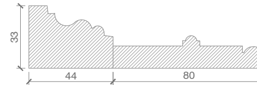
TYP. ARCHITRAVE DETAIL HIERARCHY 1 REGENCY PERIOD SCALE - 1:2
