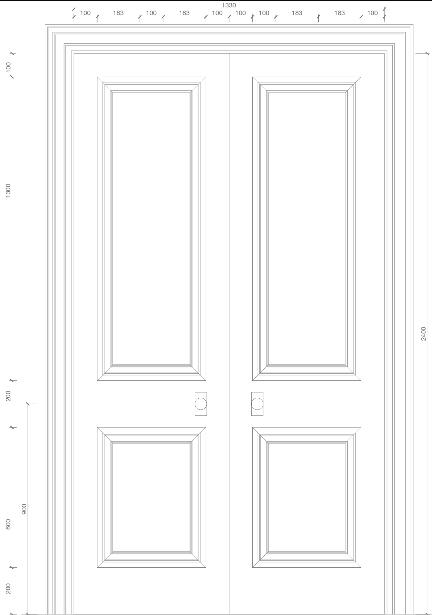
DOOR REF. DG-02, (FD30) REGENCY PERIOD, TWO PANEL SLIDING DOOR
