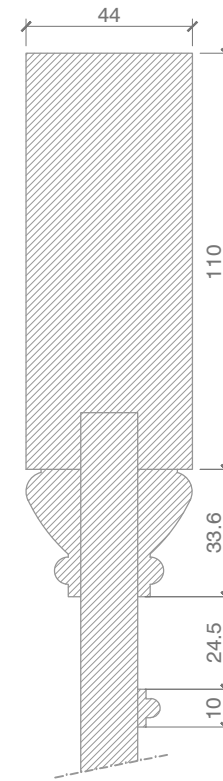
DOOR PROFILE DETAIL FOR DG-02 HIERARCHY 1 REGENCY FOUR PANEL DOOR SCALE - 1:2
