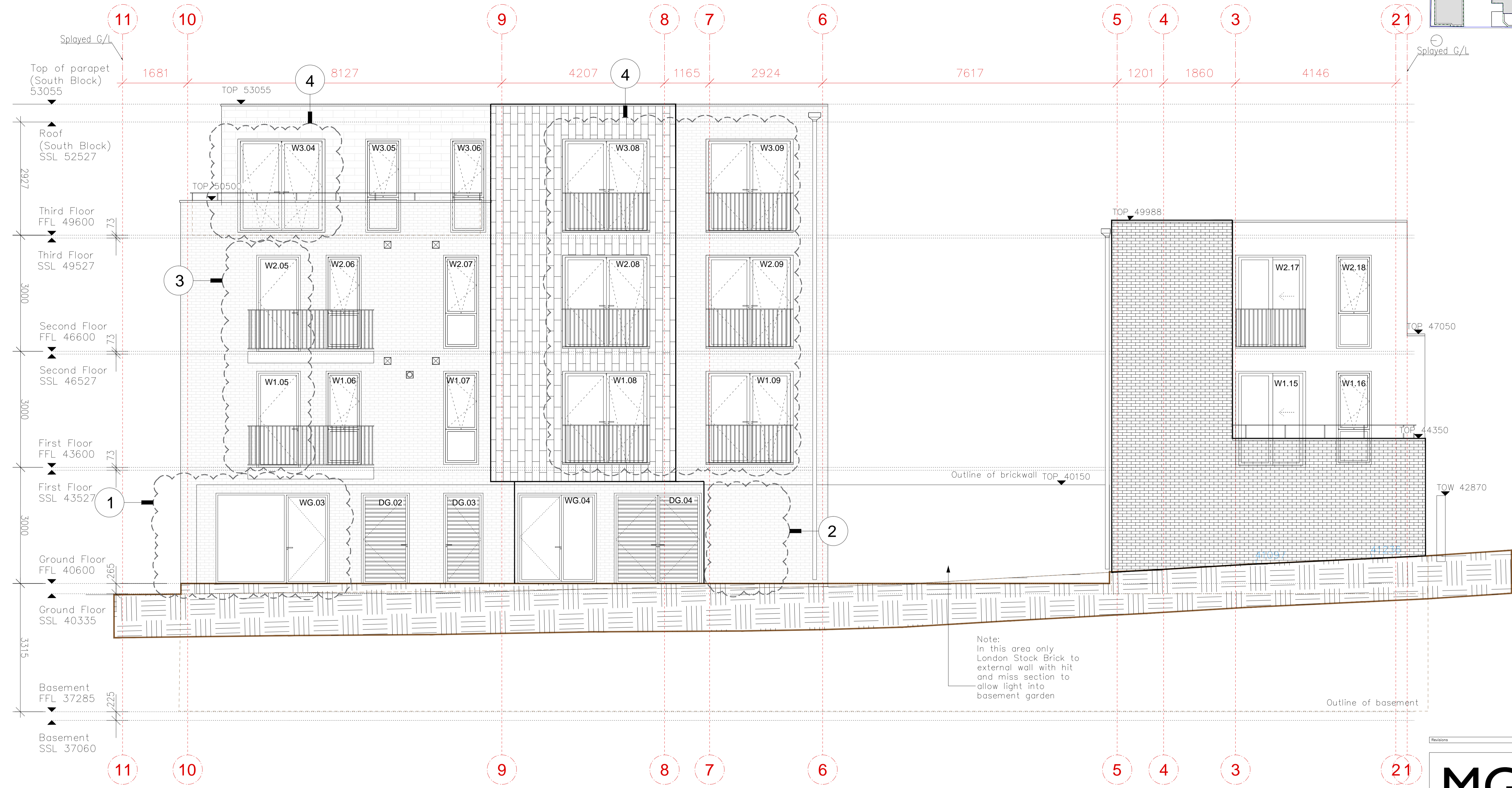
East Elevation SCALE 1:50@A1
