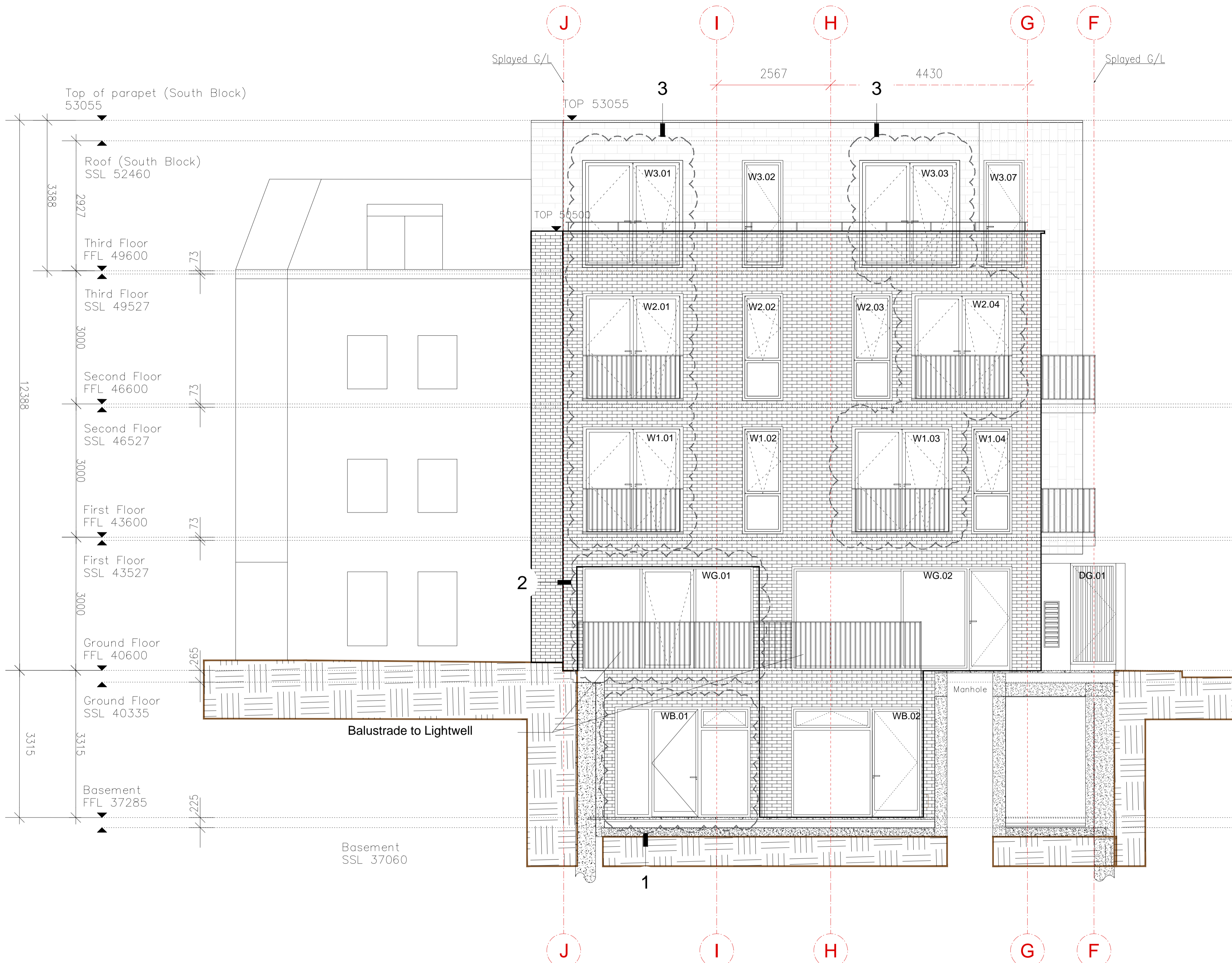
South Elevation SCALE 1:50@A1
