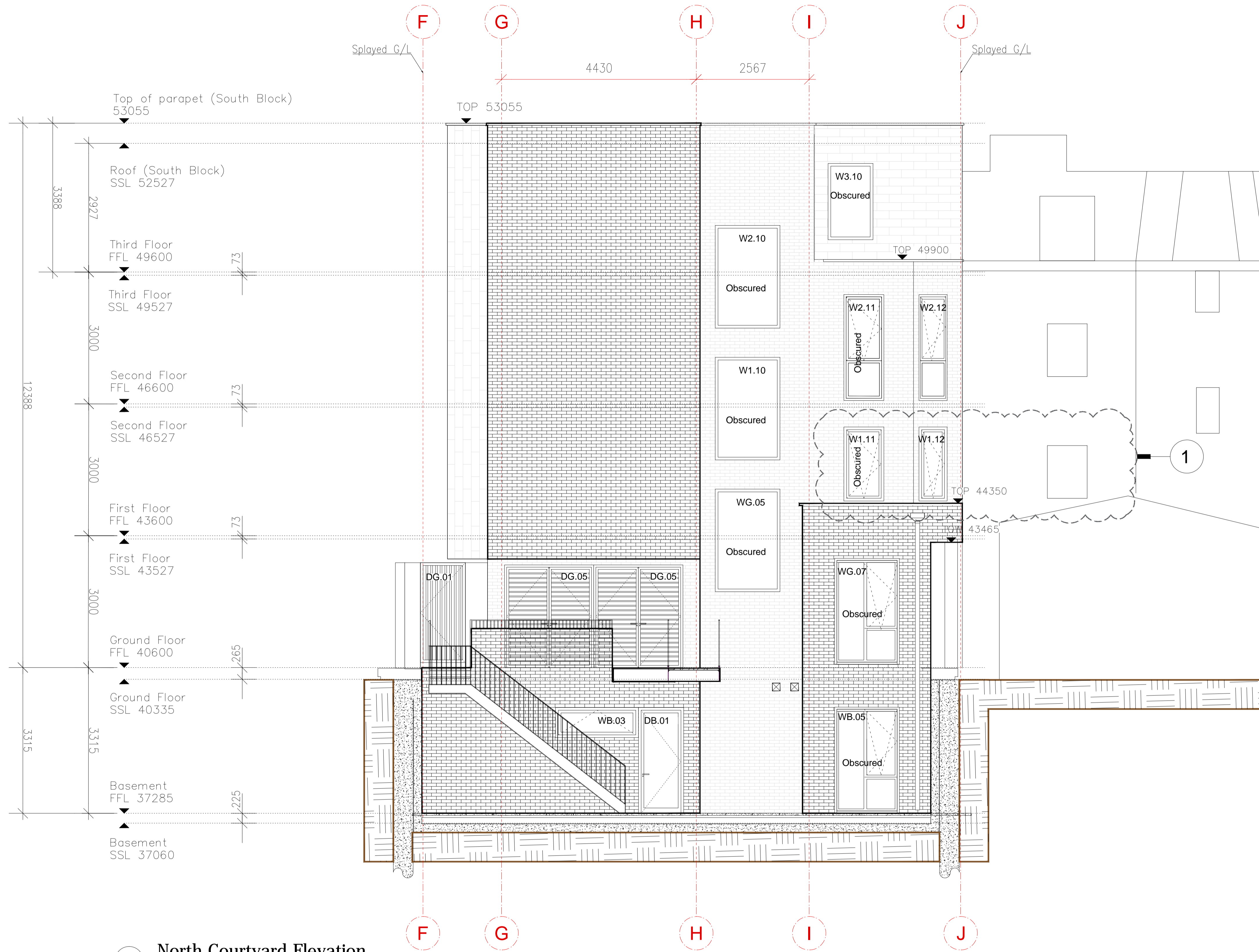
North Courtyard Elevation SCALE 1:50@A1
