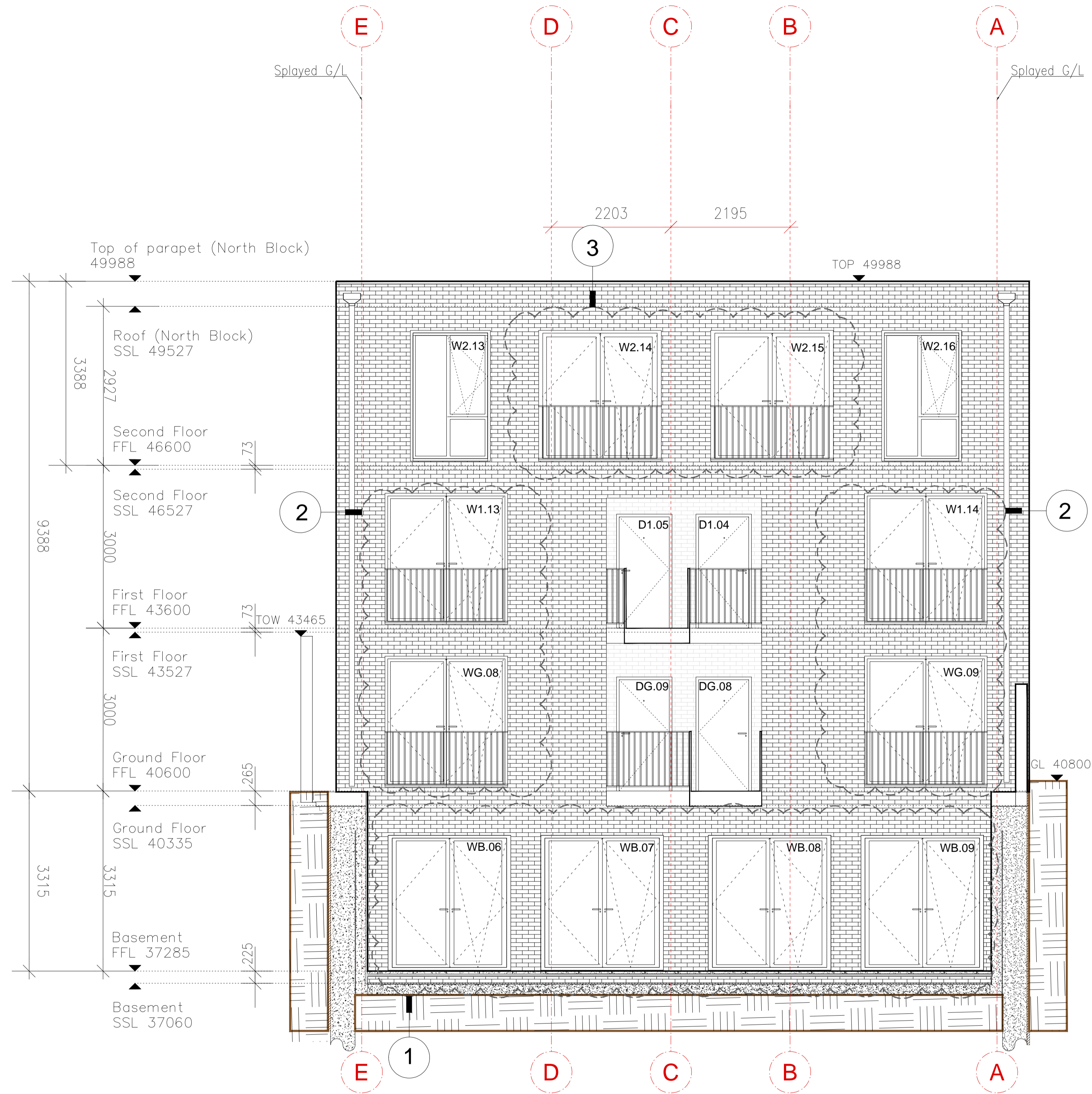
South Courtyard Elevation SCALE 1:50@A1
