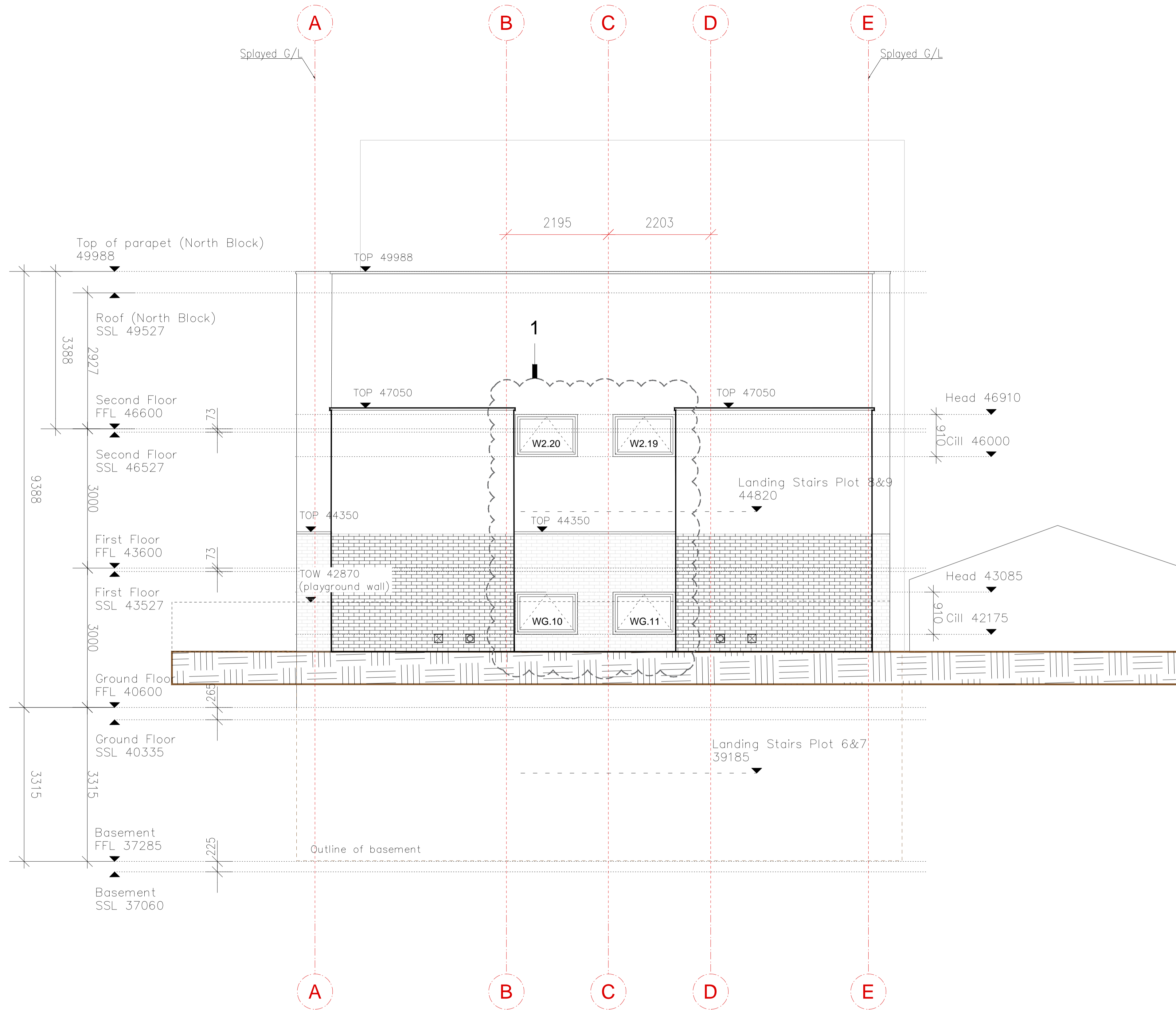
North Elevation SCALE 1:50@A1
