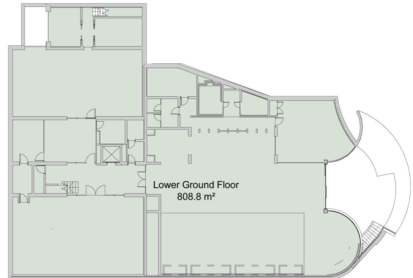
4 LOWER GROUND FLOOR LEVEL 1 : 250 @ A3
