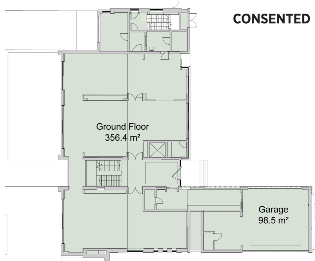
3 GROUND FLOOR LEVEL 1 : 250 @ A3
