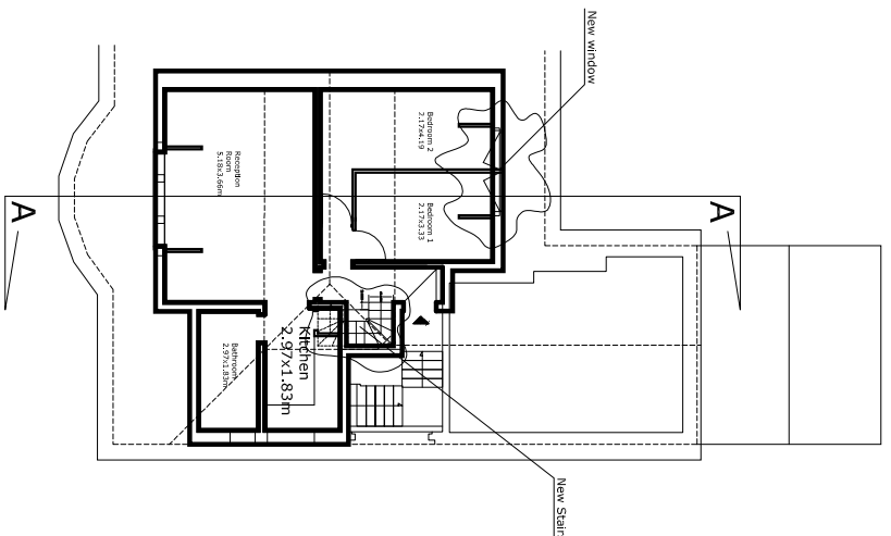
2nd Floor Plan Scale: 1/200
