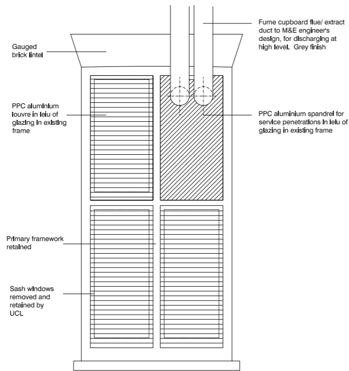
2 Gower Court West Proposed First Flr Plant Room Window Elevation SCALE 1:20@A1
