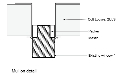
3 Gower Court West First Flr Plant Room Window Existing Framework & Louvre Junction Detail (Contractor Proposal)
