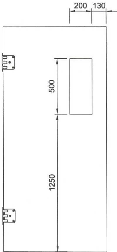
VISION PANEL SIZE FOR DOUBLE SWING DOORS
